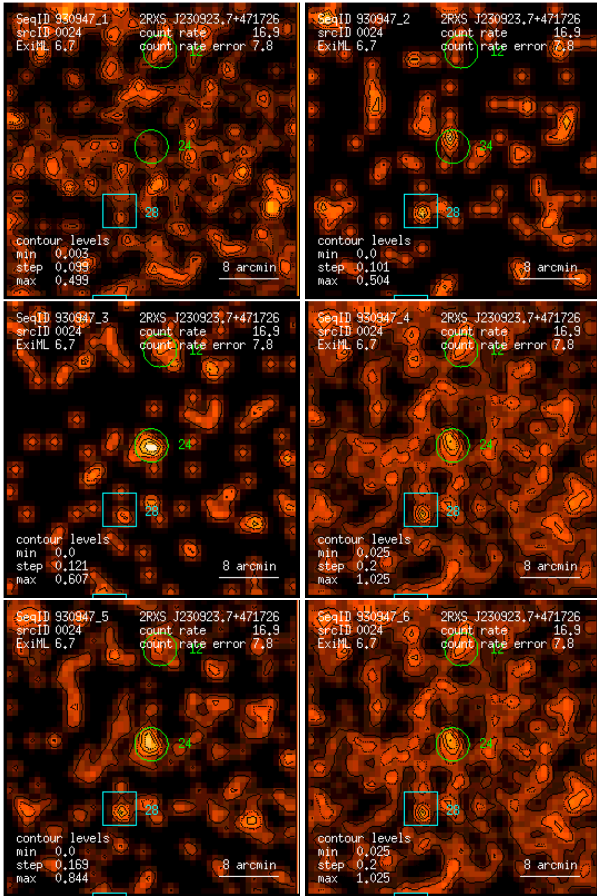
Figure 24: RASS 930947: detection 0024: band rate images, Gaussian filter: (1) PSPC channels 11 – 41, (2) 52 – 90, (3) 91 – 201, (4) 11 – 235, (5) 52 – 201, (6) 11 – 201. Broad band rates in counts/ks. Band rate contour levels in counts/ks/arcmin 2 .
