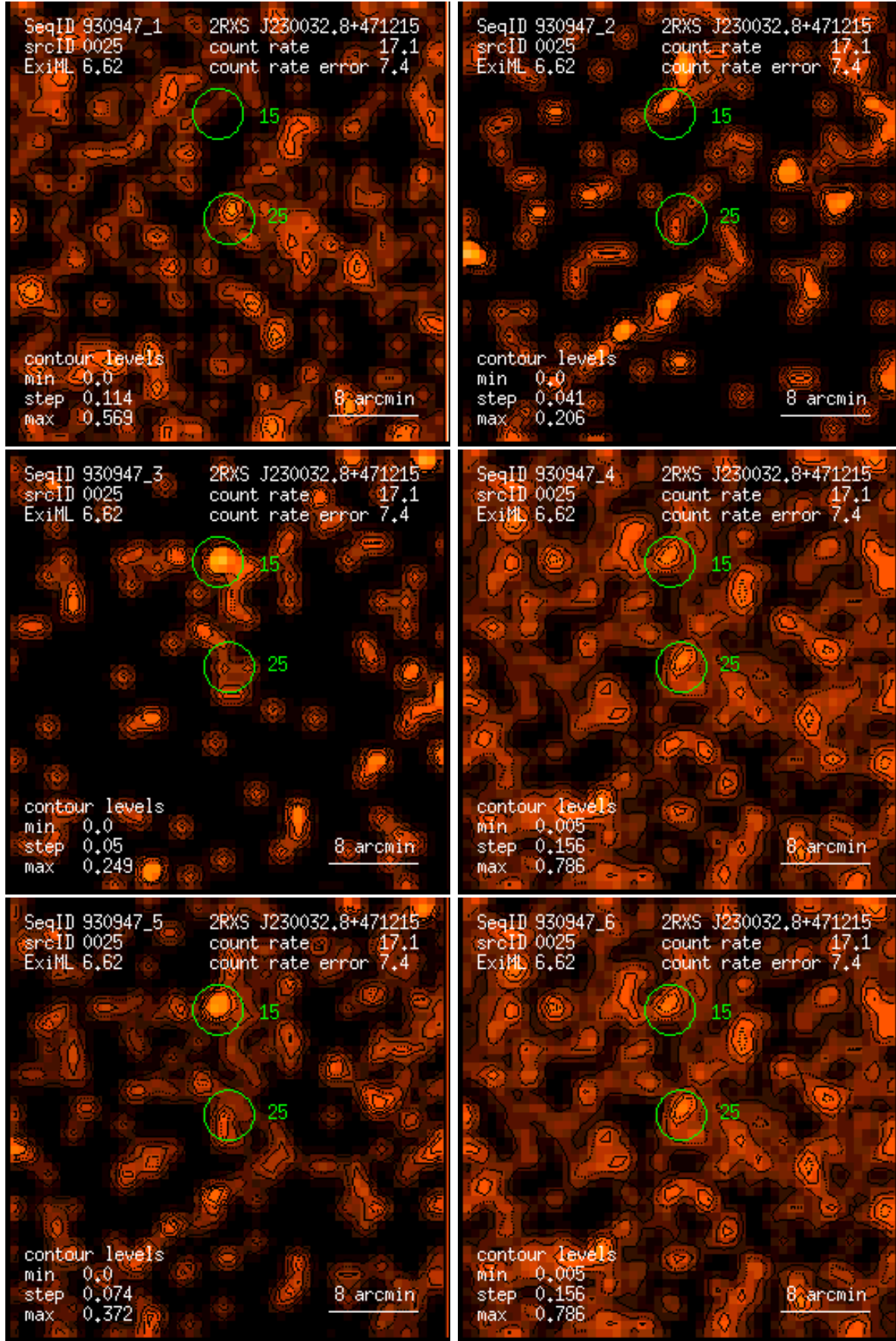
Figure 25: RASS 930947: detection 0025: band rate images, Gaussian filter: (1) PSPC channels 11 – 41, (2) 52 – 90, (3) 91 – 201, (4) 11 – 235, (5) 52 – 201, (6) 11 – 201. Broad band rates in counts/ks. Band rate contour levels in counts/ks/arcmin 2 .
