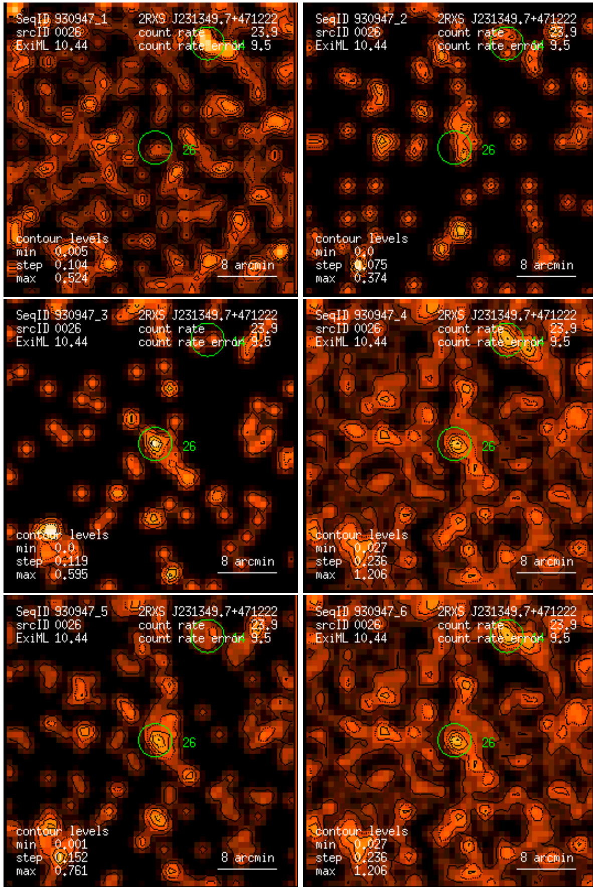
Figure 26: RASS 930947: detection 0026: band rate images, Gaussian filter: (1) PSPC channels 11 – 41, (2) 52 – 90, (3) 91 – 201, (4) 11 – 235, (5) 52 – 201, (6) 11 – 201. Broad band rates in counts/ks. Band rate contour levels in counts/ks/arcmin 2 .
