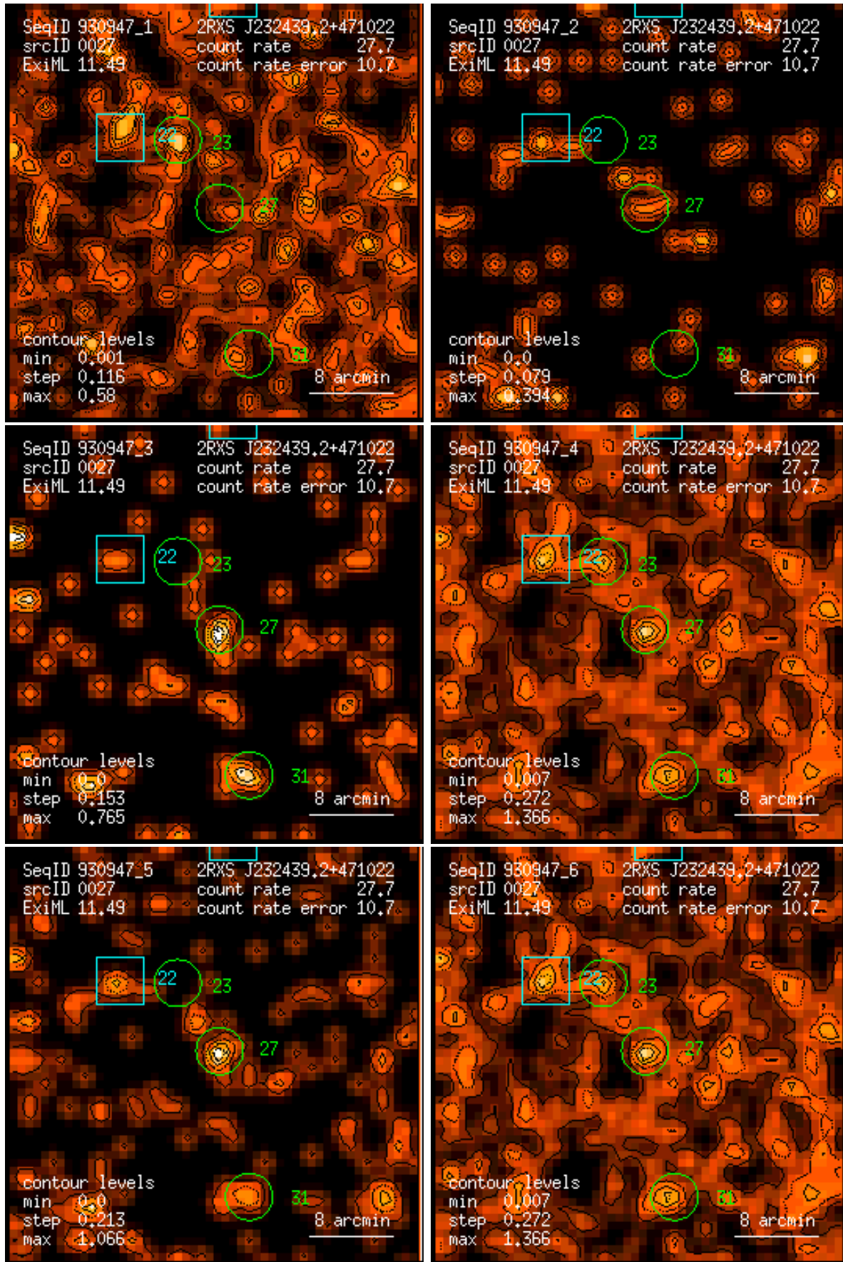
Figure 27: RASS 930947: detection 0027: band rate images, Gaussian filter: (1) PSPC channels 11 – 41, (2) 52 – 90, (3) 91 – 201, (4) 11 – 235, (5) 52 – 201, (6) 11 – 201. Broad band rates in counts/ks. Band rate contour levels in counts/ks/arcmin 2 .
