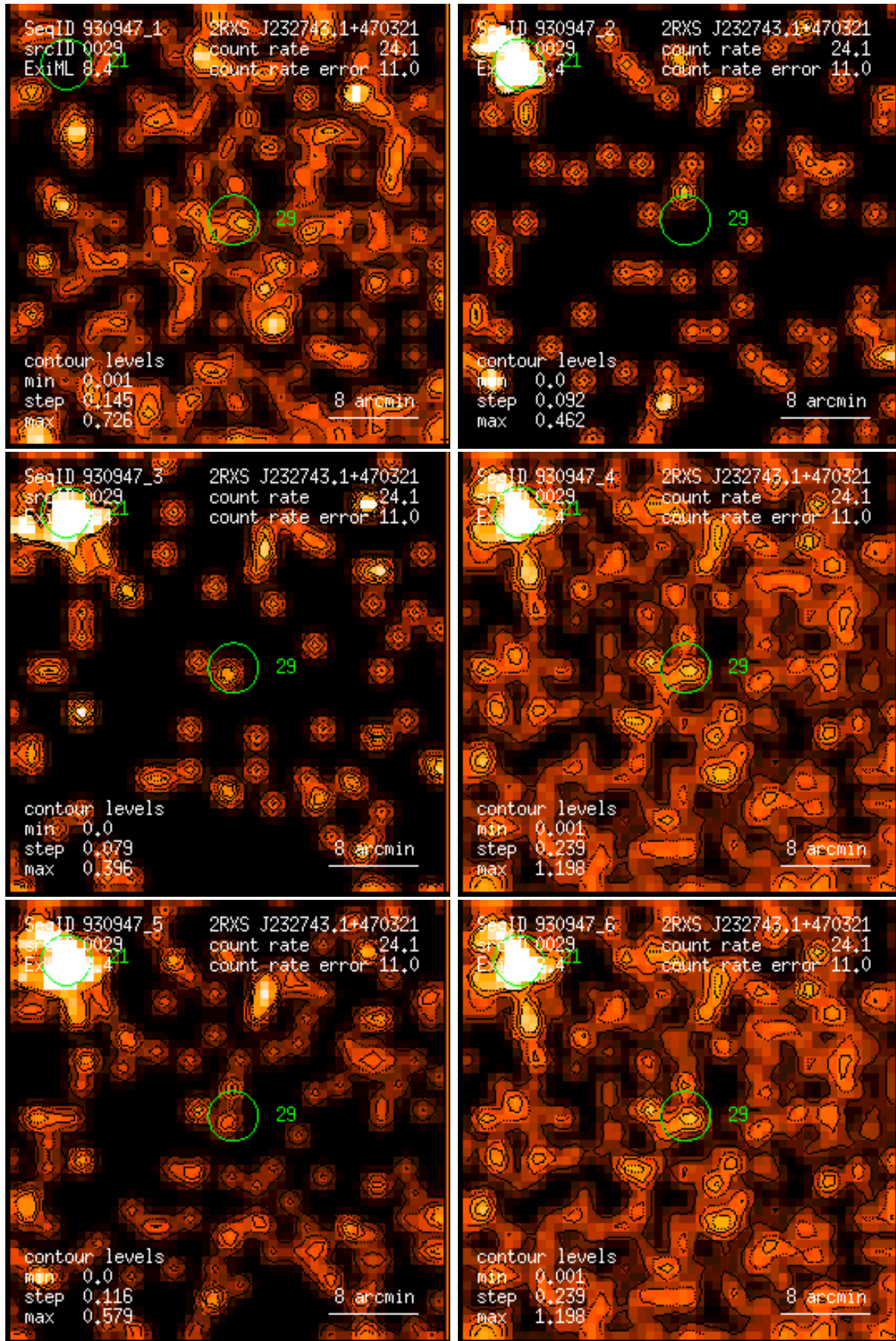
Figure 29: RASS 930947: detection 0029: band rate images, Gaussian filter: (1) PSPC channels 11 – 41, (2) 52 – 90, (3) 91 – 201, (4) 11 – 235, (5) 52 – 201, (6) 11 – 201. Broad band rates in counts/ks. Band rate contour levels in counts/ks/arcmin 2 .
