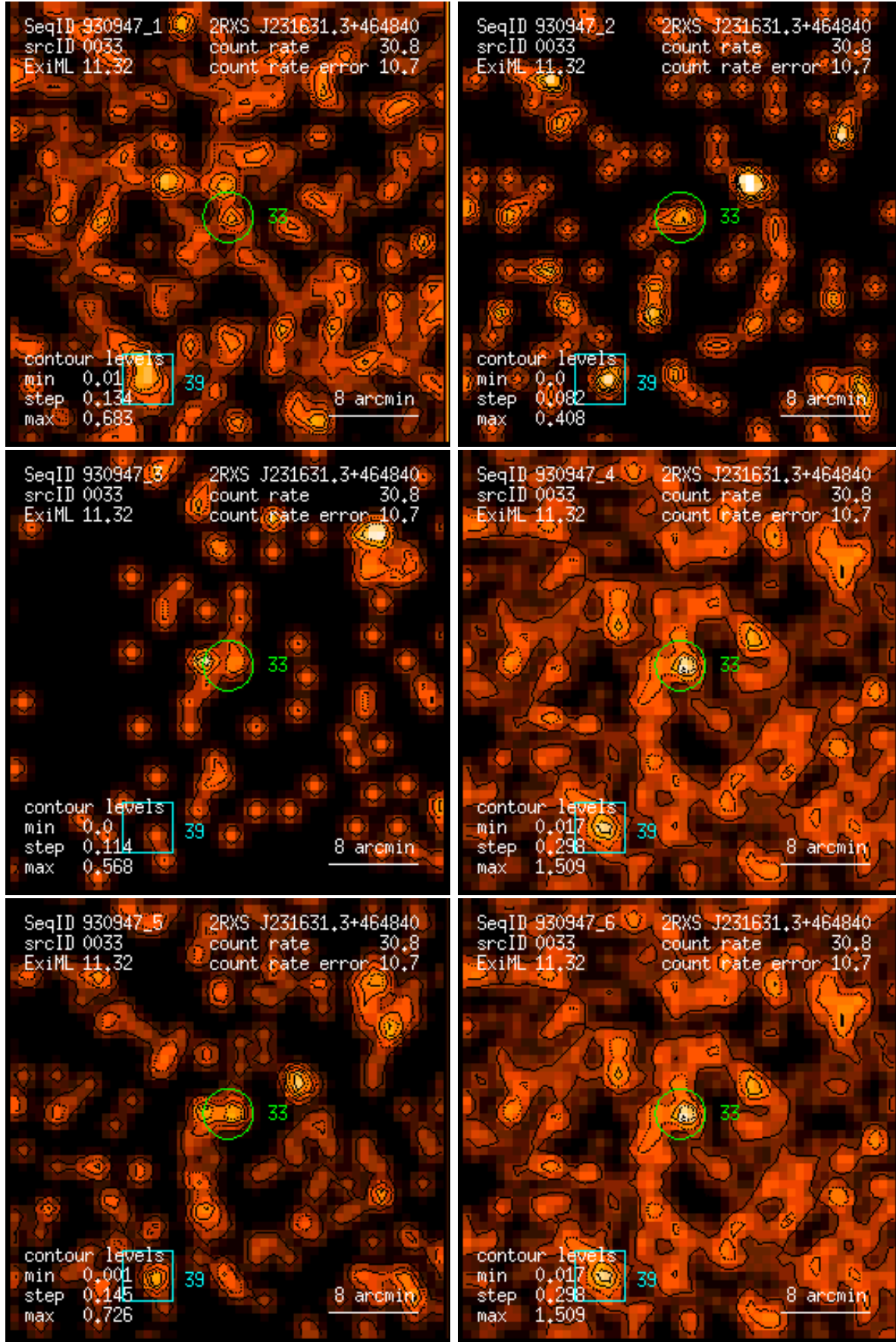
Figure 33: RASS 930947: detection 0033: band rate images, Gaussian filter: (1) PSPC channels 11 – 41, (2) 52 – 90, (3) 91 – 201, (4) 11 – 235, (5) 52 – 201, (6) 11 – 201. Broad band rates in counts/ks. Band rate contour levels in counts/ks/arcmin 2 .
