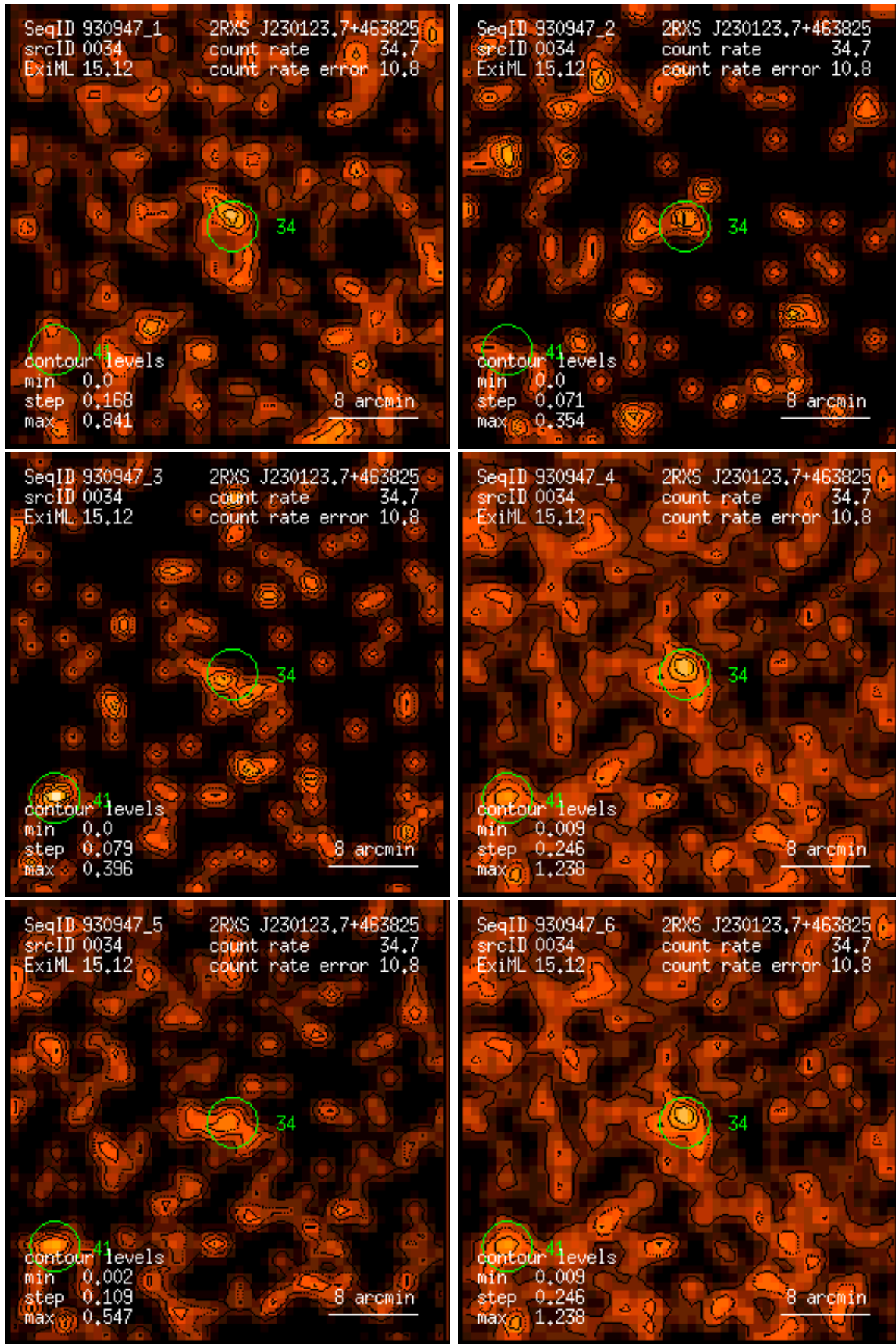
Figure 34: RASS 930947: detection 0034: band rate images, Gaussian filter: (1) PSPC channels 11 – 41, (2) 52 – 90, (3) 91 – 201, (4) 11 – 235, (5) 52 – 201, (6) 11 – 201. Broad band rates in counts/ks. Band rate contour levels in counts/ks/arcmin 2 .
