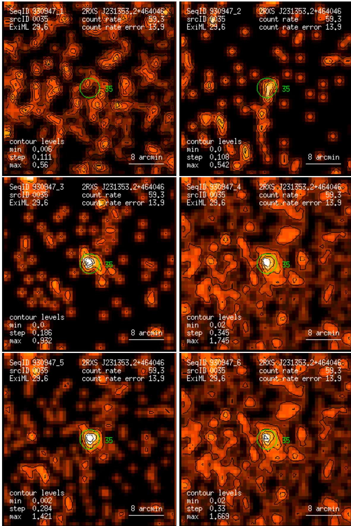
Figure 35: RASS 930947: detection 0035: band rate images, Gaussian filter: (1) PSPC channels 11 – 41, (2) 52 – 90, (3) 91 – 201, (4) 11 – 235, (5) 52 – 201, (6) 11 – 201. Broad band rates in counts/ks. Band rate contour levels in counts/ks/arcmin 2 .
