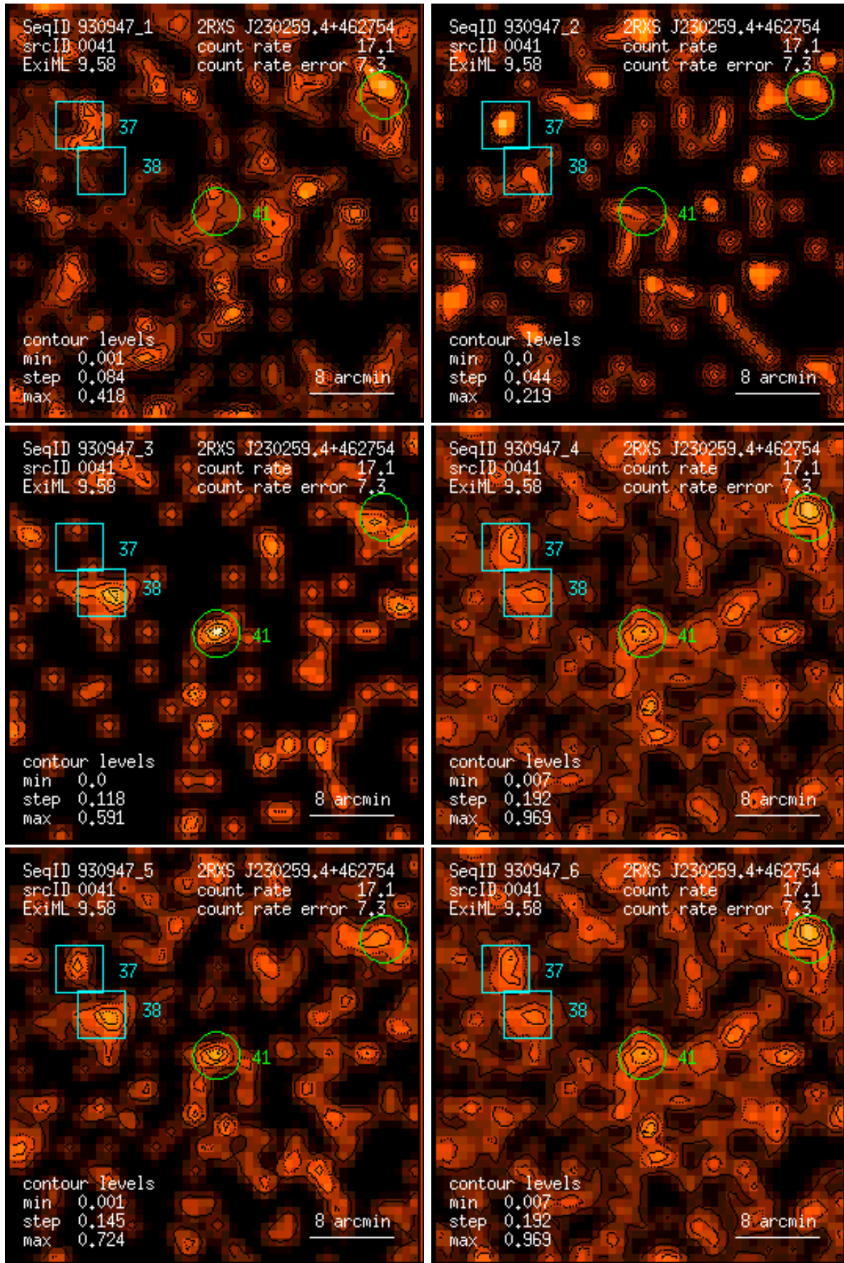
Figure 41: RASS 930947: detection 0041: band rate images, Gaussian filter: (1) PSPC channels 11 – 41, (2) 52 – 90, (3) 91 – 201, (4) 11 – 235, (5) 52 – 201, (6) 11 – 201. Broad band rates in counts/ks. Band rate contour levels in counts/ks/arcmin 2 .
