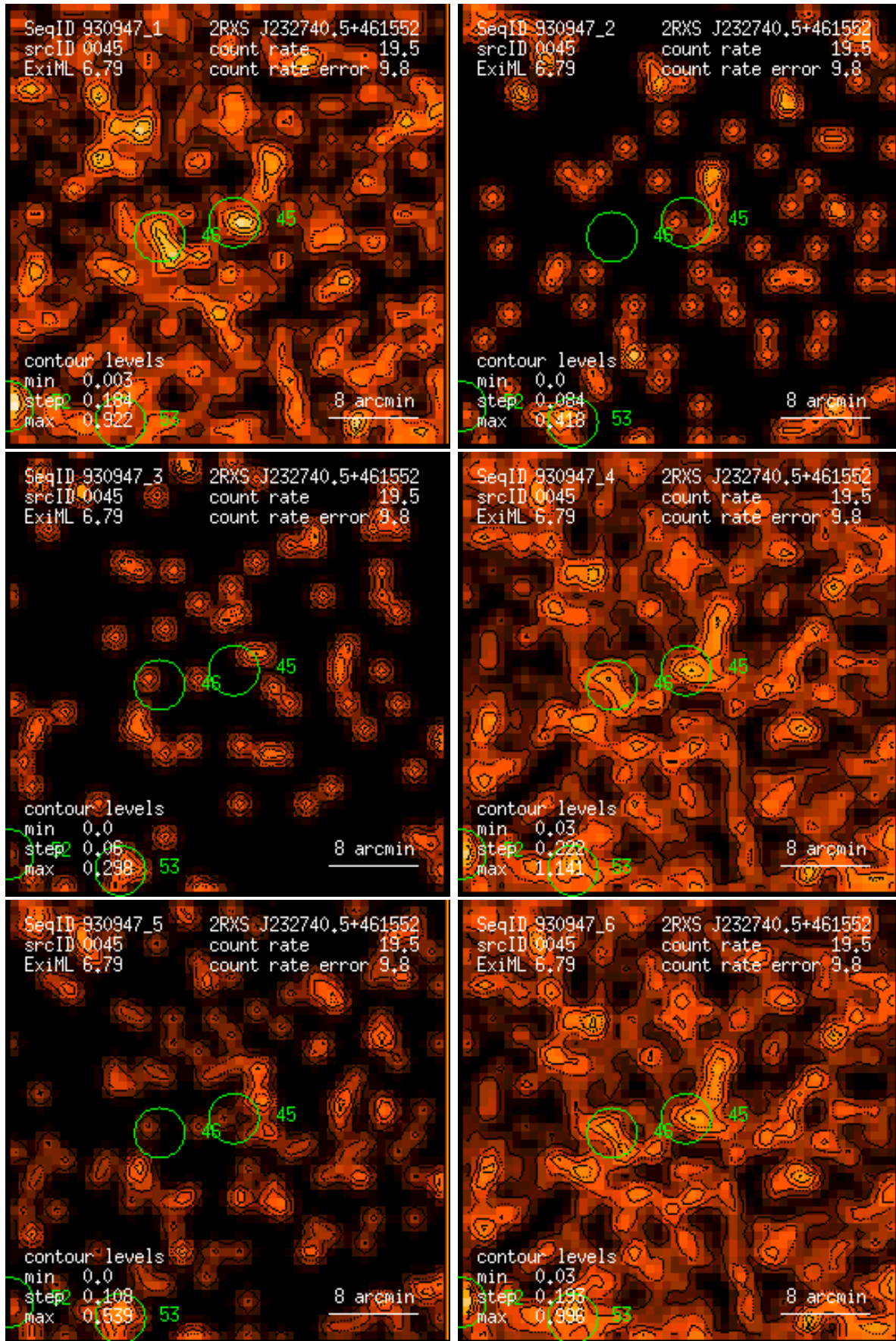
Figure 45: RASS 930947: detection 0045: band rate images, Gaussian filter: (1) PSPC channels 11 – 41, (2) 52 – 90, (3) 91 – 201, (4) 11 – 235, (5) 52 – 201, (6) 11 – 201. Broad band rates in counts/ks. Band rate contour levels in counts/ks/arcmin 2 .
