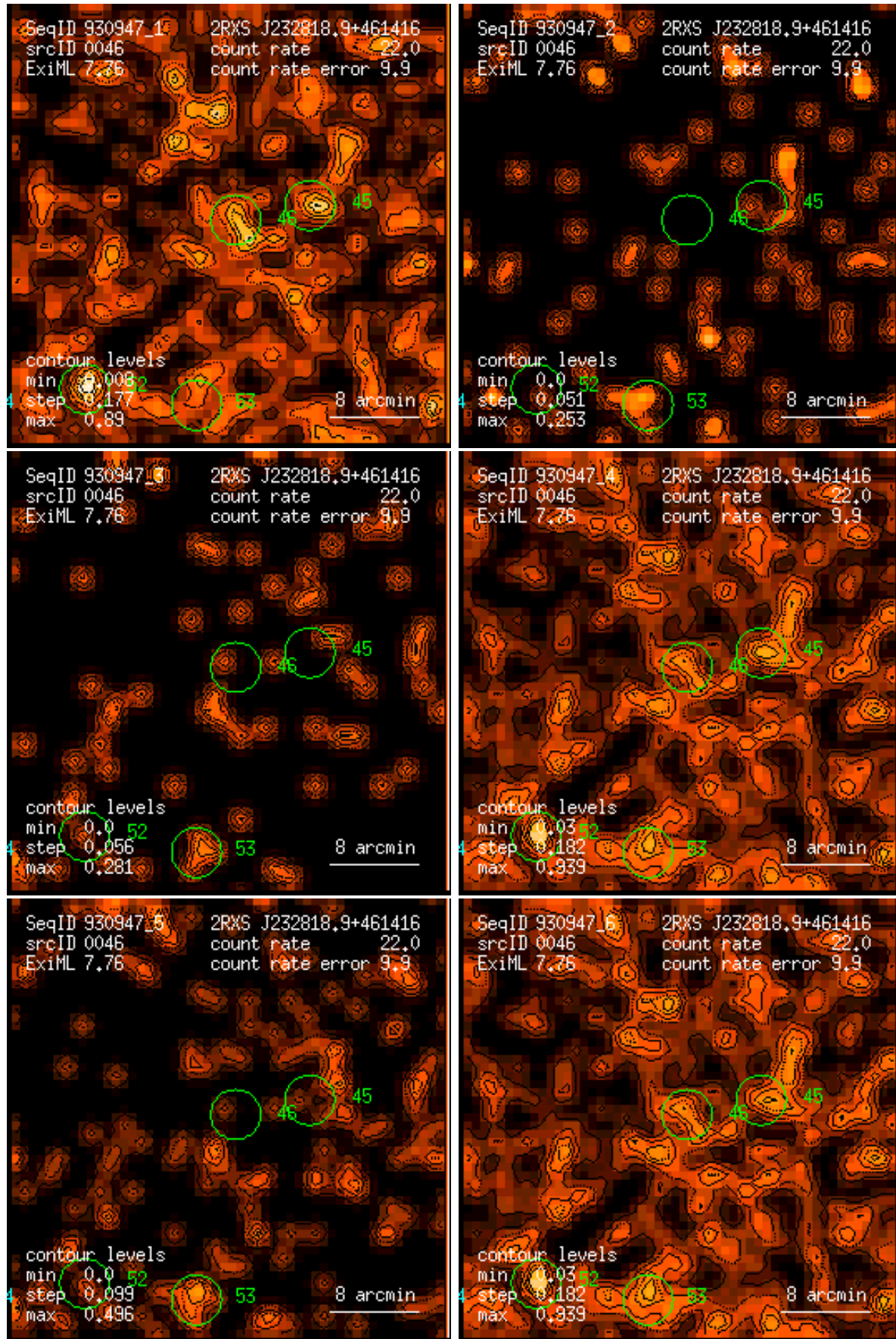
Figure 46: RASS 930947: detection 0046: band rate images, Gaussian filter: (1) PSPC channels 11 – 41, (2) 52 – 90, (3) 91 – 201, (4) 11 – 235, (5) 52 – 201, (6) 11 – 201. Broad band rates in counts/ks. Band rate contour levels in counts/ks/arcmin 2 .
