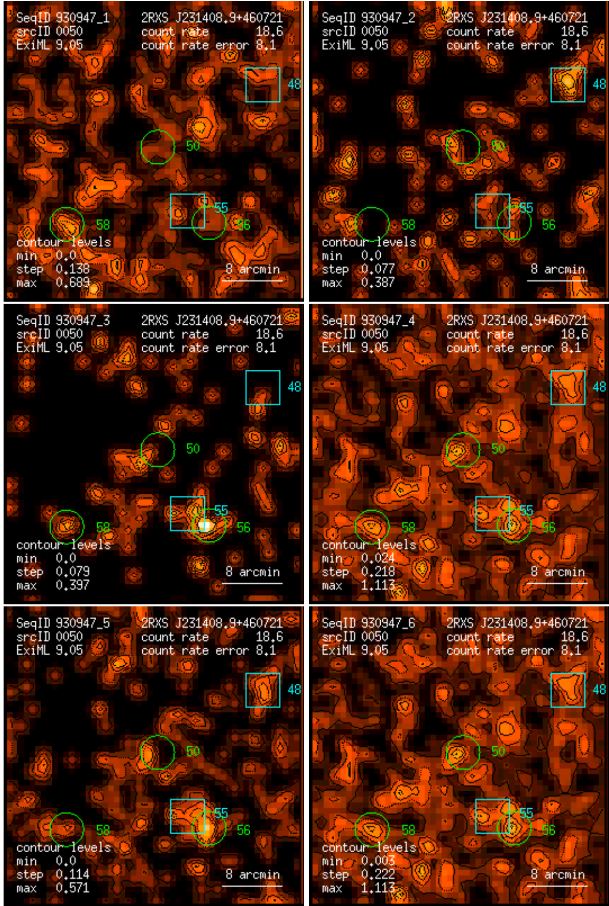
Figure 50: RASS 930947: detection 0050: band rate images, Gaussian filter: (1) PSPC channels 11 – 41, (2) 52 – 90, (3) 91 – 201, (4) 11 – 235, (5) 52 – 201, (6) 11 – 201. Broad band rates in counts/ks. Band rate contour levels in counts/ks/arcmin 2 .
