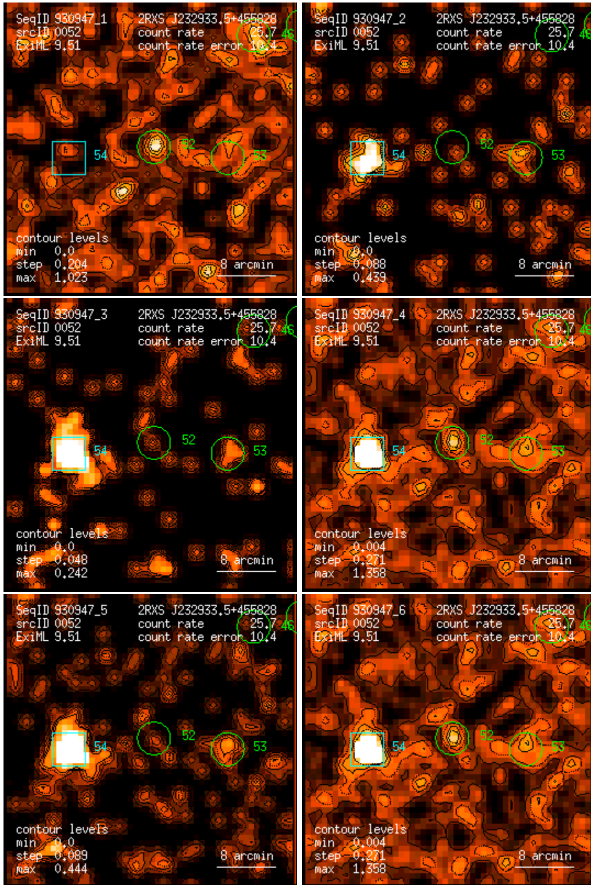
Figure 52: RASS 930947: detection 0052: band rate images, Gaussian filter: (1) PSPC channels 11 – 41, (2) 52 – 90, (3) 91 – 201, (4) 11 – 235, (5) 52 – 201, (6) 11 – 201. Broad band rates in counts/ks. Band rate contour levels in counts/ks/arcmin 2 .
