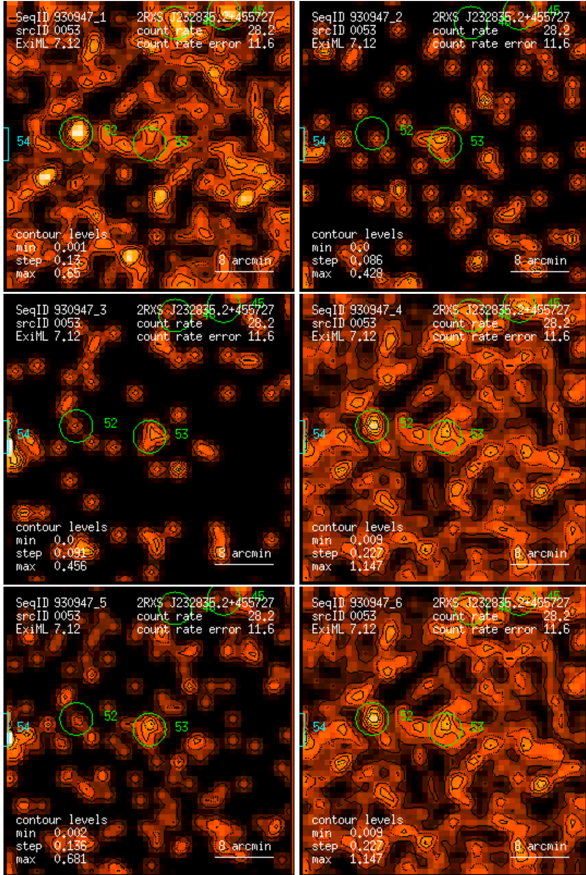
Figure 53: RASS 930947: detection 0053: band rate images, Gaussian filter: (1) PSPC channels 11 – 41, (2) 52 – 90, (3) 91 – 201, (4) 11 – 235, (5) 52 – 201, (6) 11 – 201. Broad band rates in counts/ks. Band rate contour levels in counts/ks/arcmin 2 .
