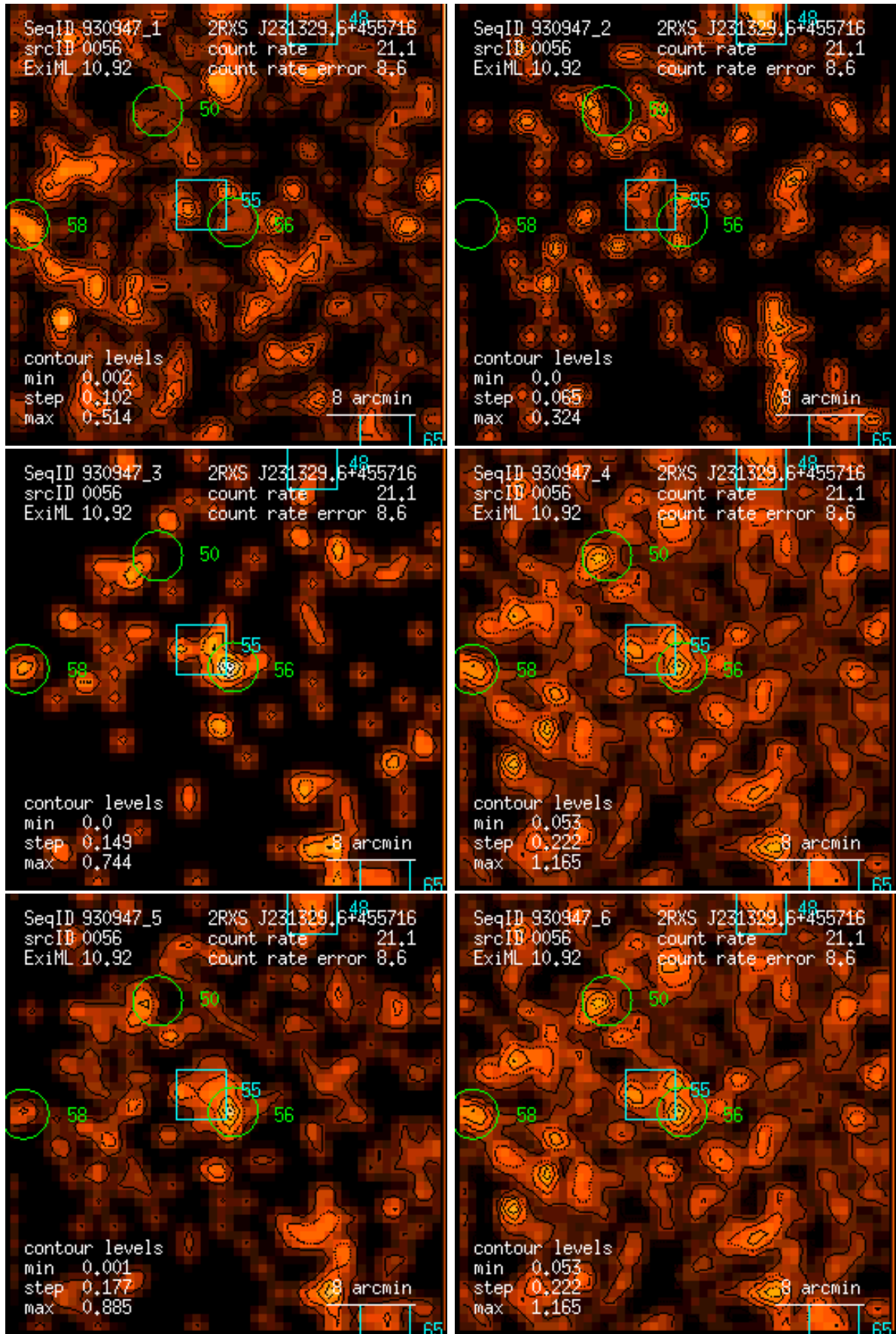
Figure 56: RASS 930947: detection 0056: band rate images, Gaussian filter: (1) PSPC channels 11 – 41, (2) 52 – 90, (3) 91 – 201, (4) 11 – 235, (5) 52 – 201, (6) 11 – 201. Broad band rates in counts/ks. Band rate contour levels in counts/ks/arcmin 2 .
