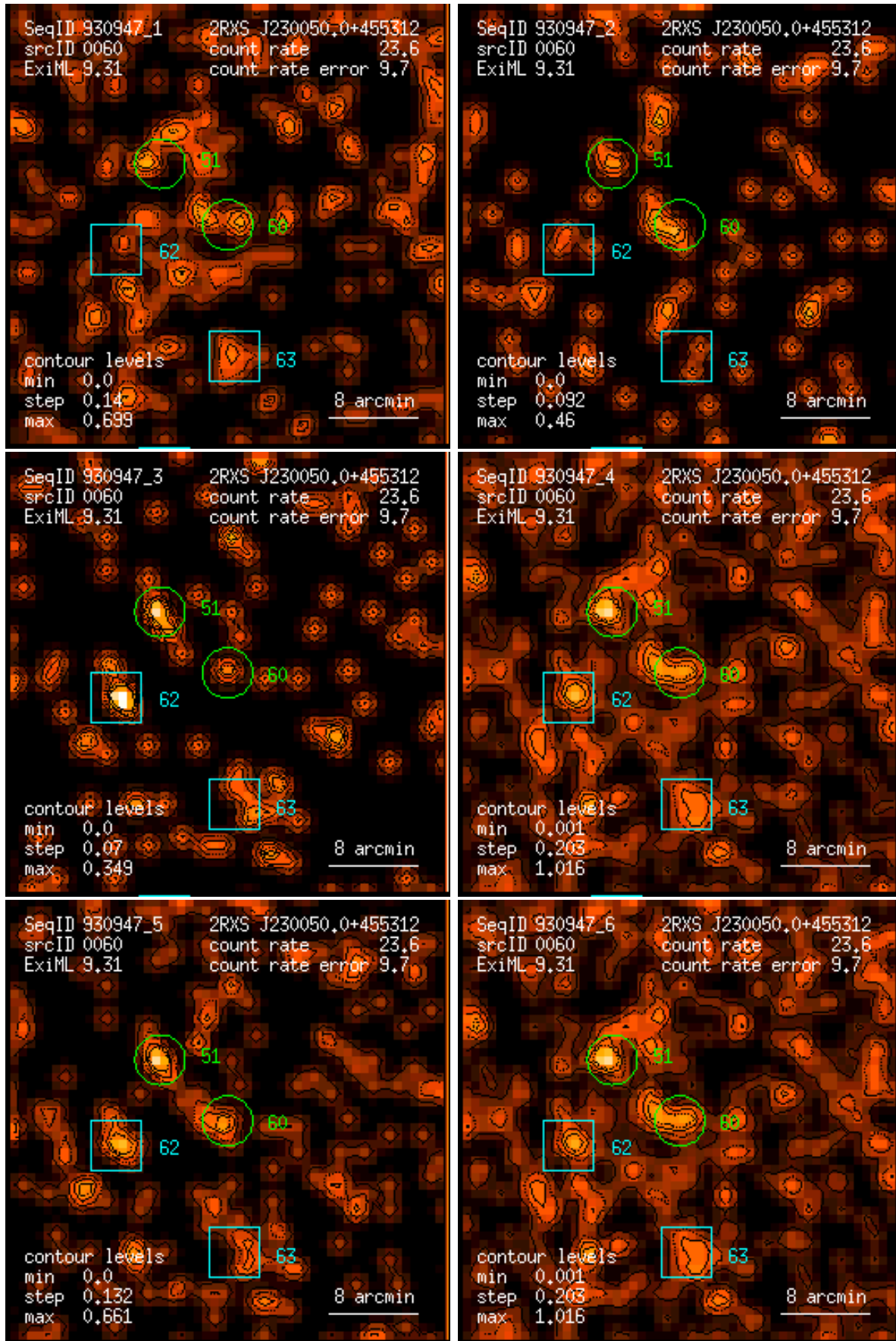
Figure 60: RASS 930947: detection 0060: band rate images, Gaussian filter: (1) PSPC channels 11 – 41, (2) 52 – 90, (3) 91 – 201, (4) 11 – 235, (5) 52 – 201, (6) 11 – 201. Broad band rates in counts/ks. Band rate contour levels in counts/ks/arcmin 2 .
