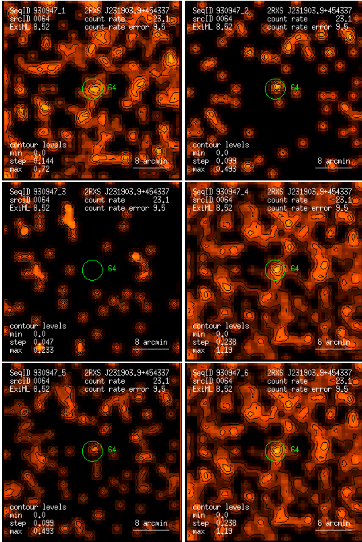
Figure 64: RASS 930947: detection 0064: band rate images, Gaussian filter: (1) PSPC channels 11 – 41, (2) 52 – 90, (3) 91 – 201, (4) 11 – 235, (5) 52 – 201, (6) 11 – 201. Broad band rates in counts/ks. Band rate contour levels in counts/ks/arcmin 2 .
