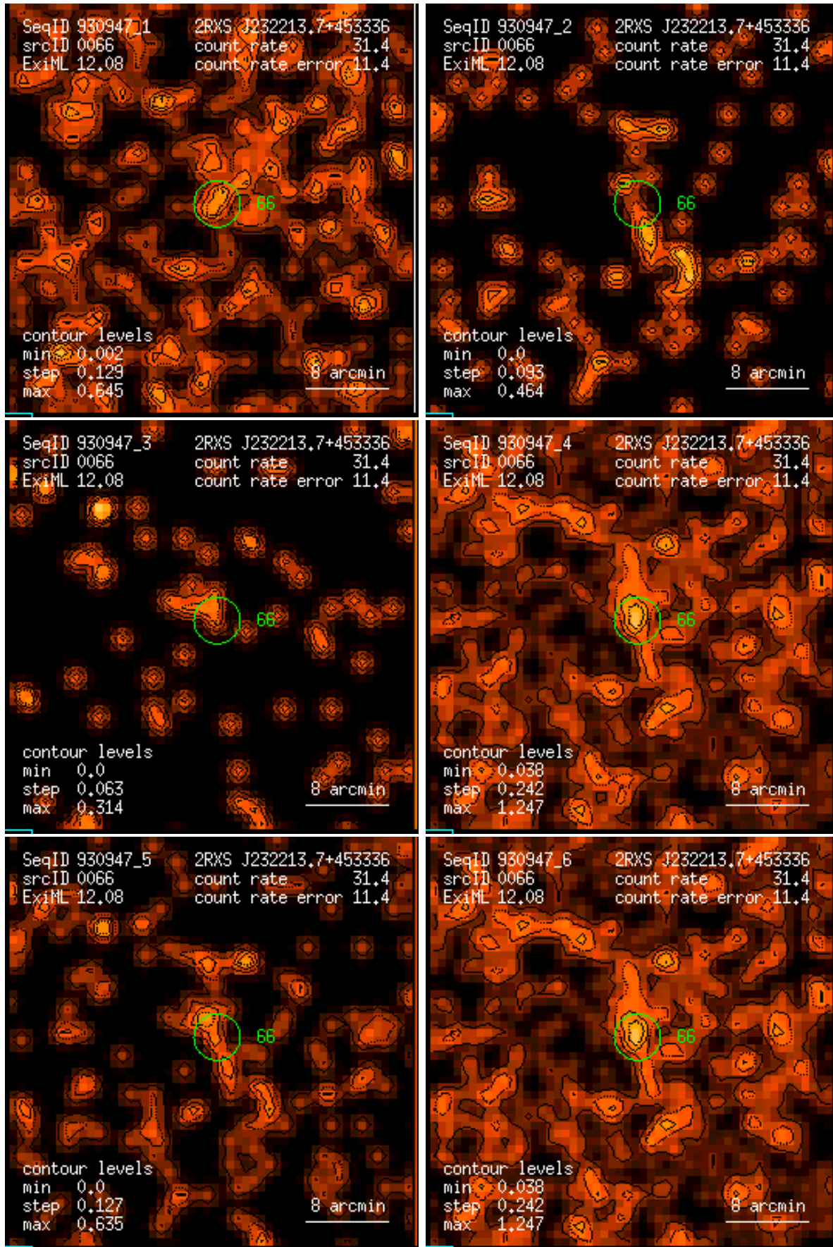
Figure 66: RASS 930947: detection 0066: band rate images, Gaussian filter: (1) PSPC channels 11 – 41, (2) 52 – 90, (3) 91 – 201, (4) 11 – 235, (5) 52 – 201, (6) 11 – 201. Broad band rates in counts/ks. Band rate contour levels in counts/ks/arcmin 2 .
