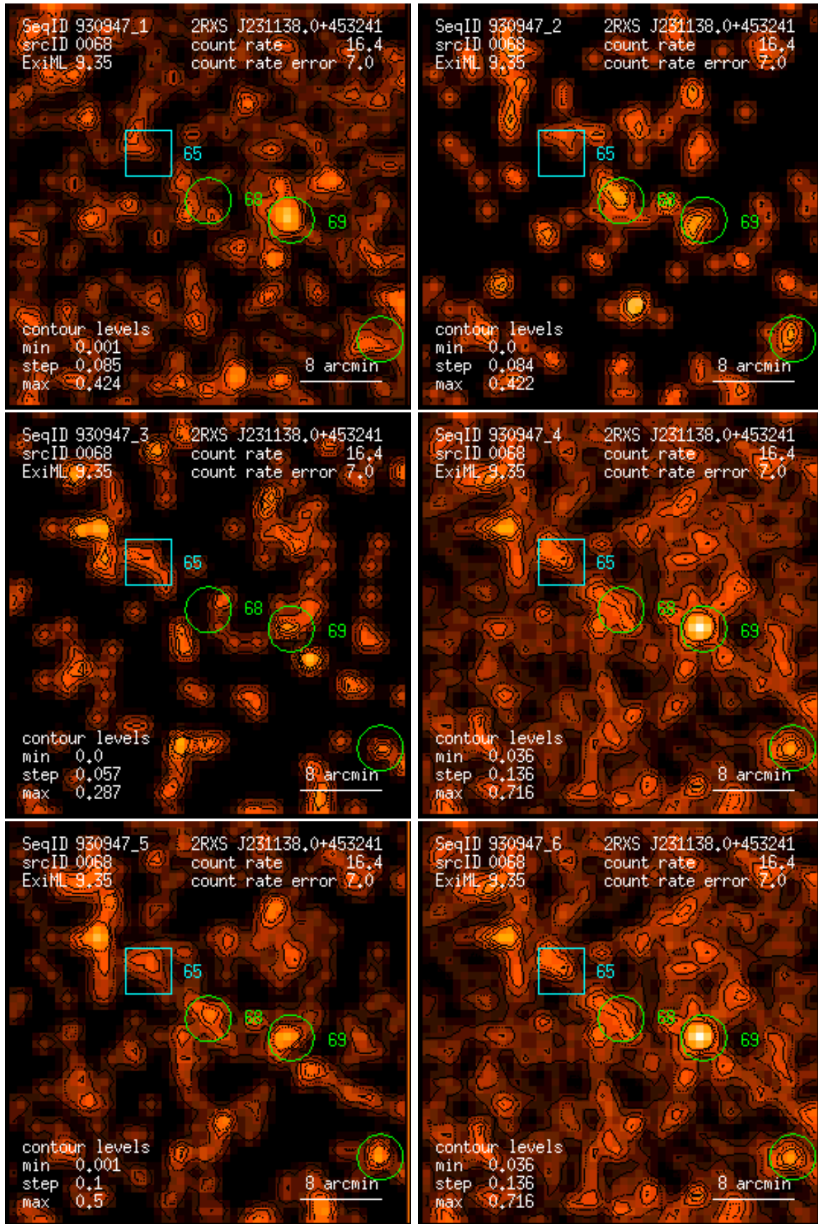
Figure 68: RASS 930947: detection 0068: band rate images, Gaussian filter: (1) PSPC channels 11 – 41, (2) 52 – 90, (3) 91 – 201, (4) 11 – 235, (5) 52 – 201, (6) 11 – 201. Broad band rates in counts/ks. Band rate contour levels in counts/ks/arcmin 2 .
