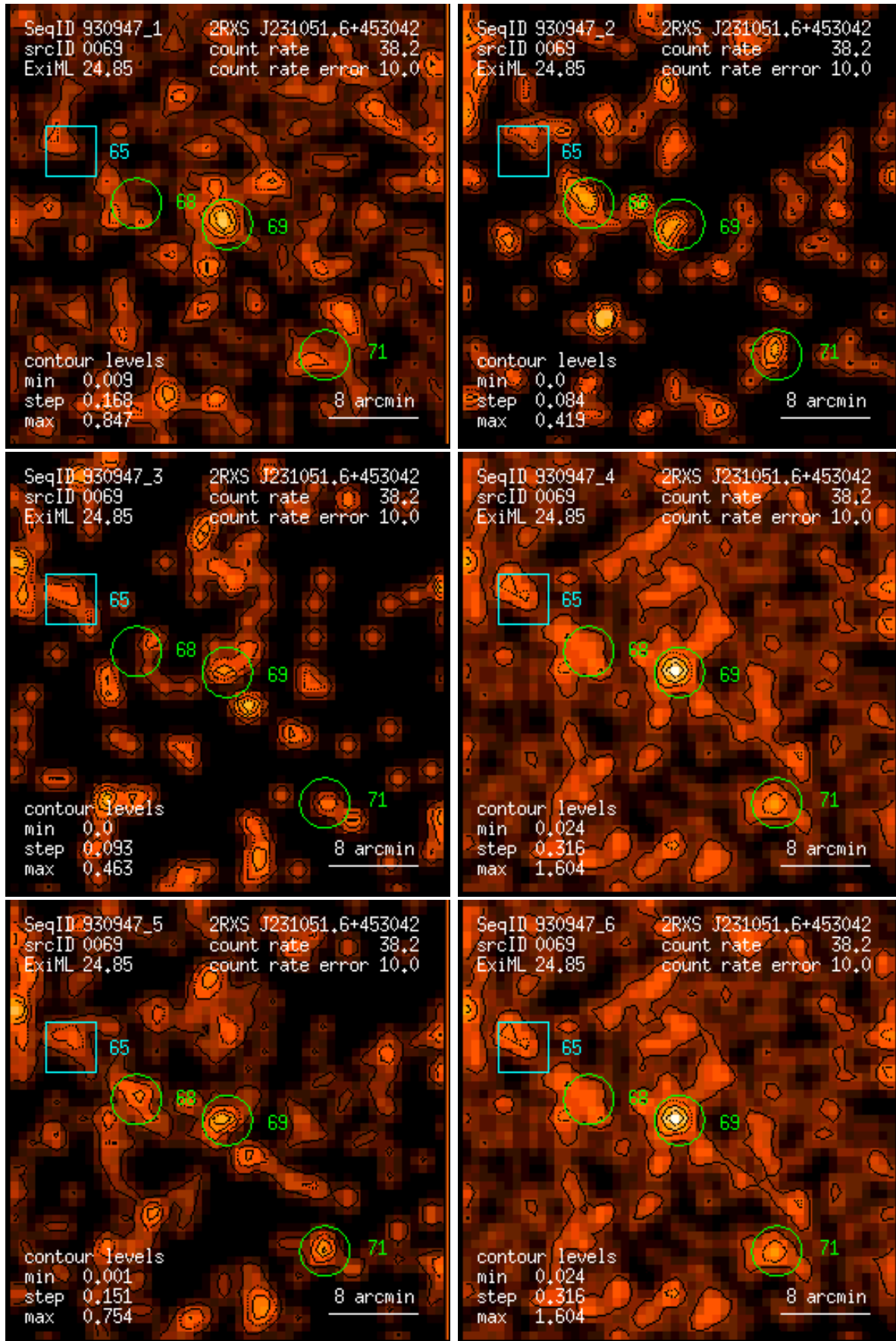
Figure 69: RASS 930947: detection 0069: band rate images, Gaussian filter: (1) PSPC channels 11 – 41, (2) 52 – 90, (3) 91 – 201, (4) 11 – 235, (5) 52 – 201, (6) 11 – 201. Broad band rates in counts/ks. Band rate contour levels in counts/ks/arcmin 2 .
