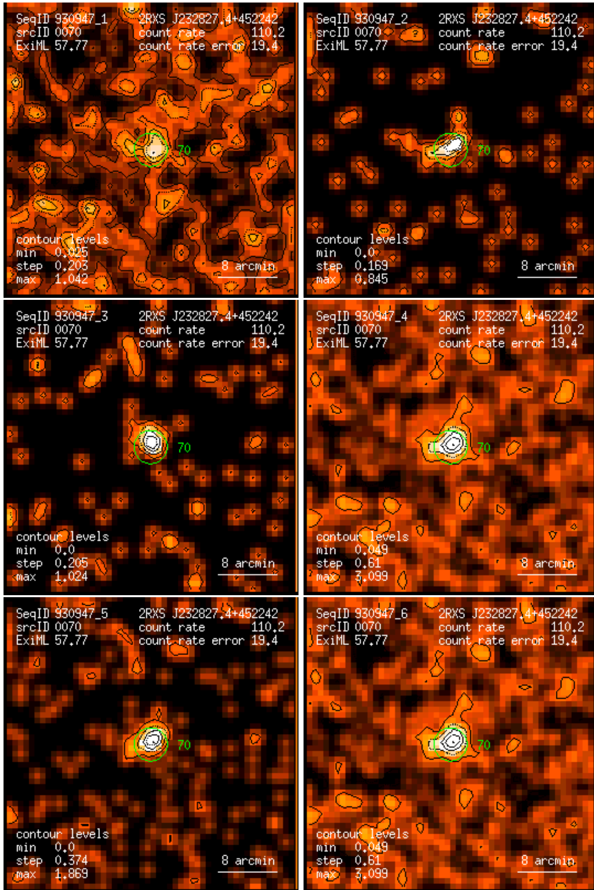
Figure 70: RASS 930947: detection 0070: band rate images, Gaussian filter: (1) PSPC channels 11 – 41, (2) 52 – 90, (3) 91 – 201, (4) 11 – 235, (5) 52 – 201, (6) 11 – 201. Broad band rates in counts/ks. Band rate contour levels in counts/ks/arcmin 2 .
