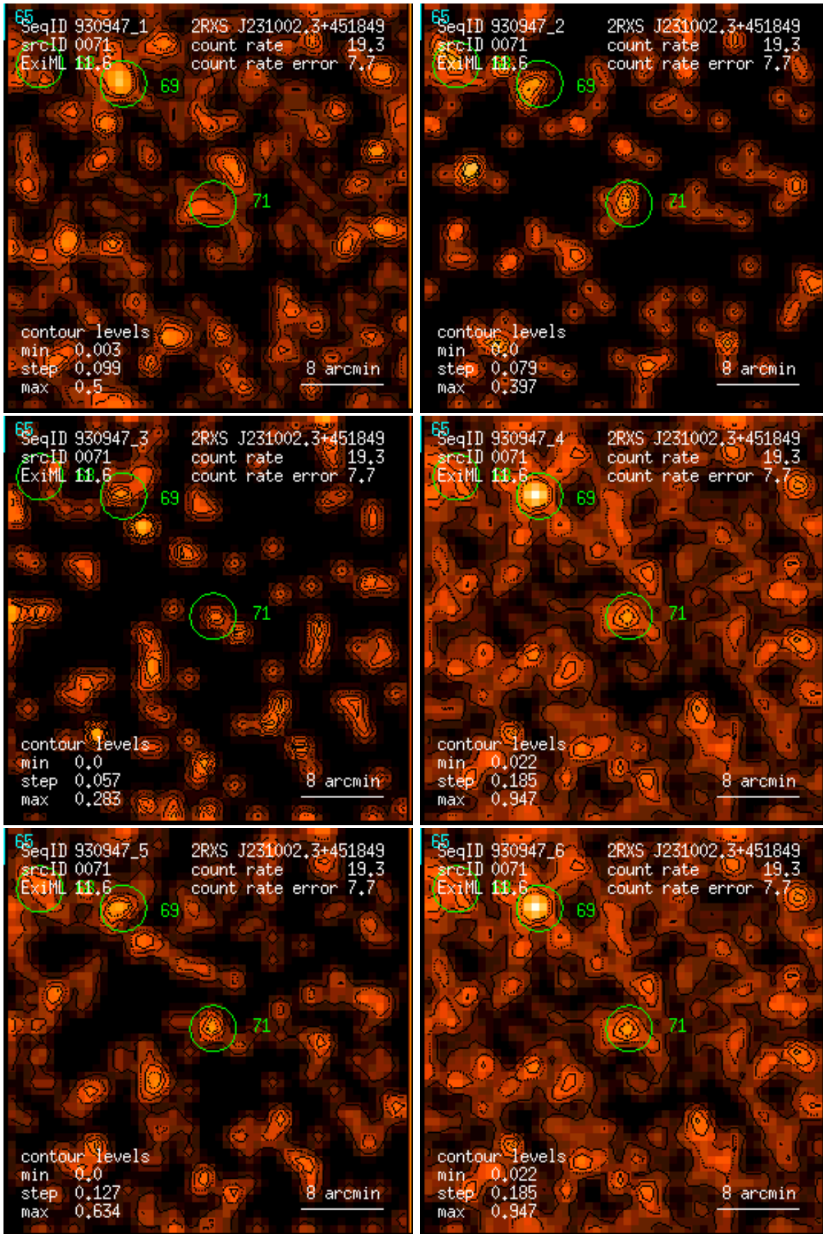
Figure 71: RASS 930947: detection 0071: band rate images, Gaussian filter: (1) PSPC channels 11 – 41, (2) 52 – 90, (3) 91 – 201, (4) 11 – 235, (5) 52 – 201, (6) 11 – 201. Broad band rates in counts/ks. Band rate contour levels in counts/ks/arcmin 2 .
