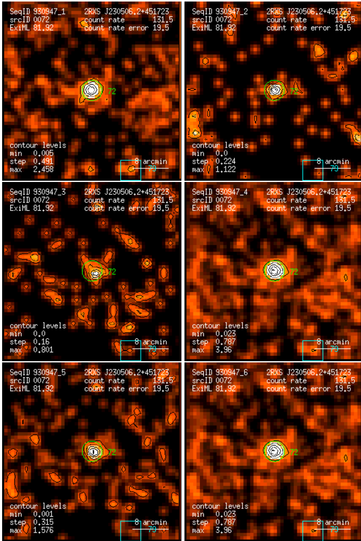
Figure 72: RASS 930947: detection 0072: band rate images, Gaussian filter: (1) PSPC channels 11 – 41, (2) 52 – 90, (3) 91 – 201, (4) 11 – 235, (5) 52 – 201, (6) 11 – 201. Broad band rates in counts/ks. Band rate contour levels in counts/ks/arcmin 2 .
