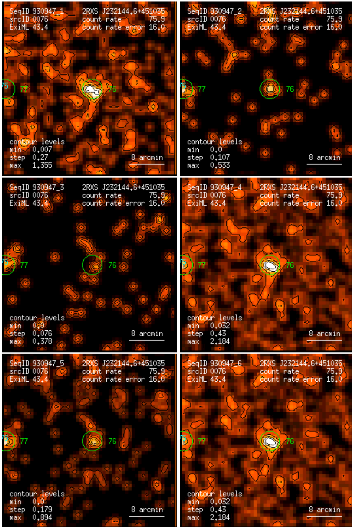
Figure 76: RASS 930947: detection 0076: band rate images, Gaussian filter: (1) PSPC channels 11 – 41, (2) 52 – 90, (3) 91 – 201, (4) 11 – 235, (5) 52 – 201, (6) 11 – 201. Broad band rates in counts/ks. Band rate contour levels in counts/ks/arcmin 2 .
