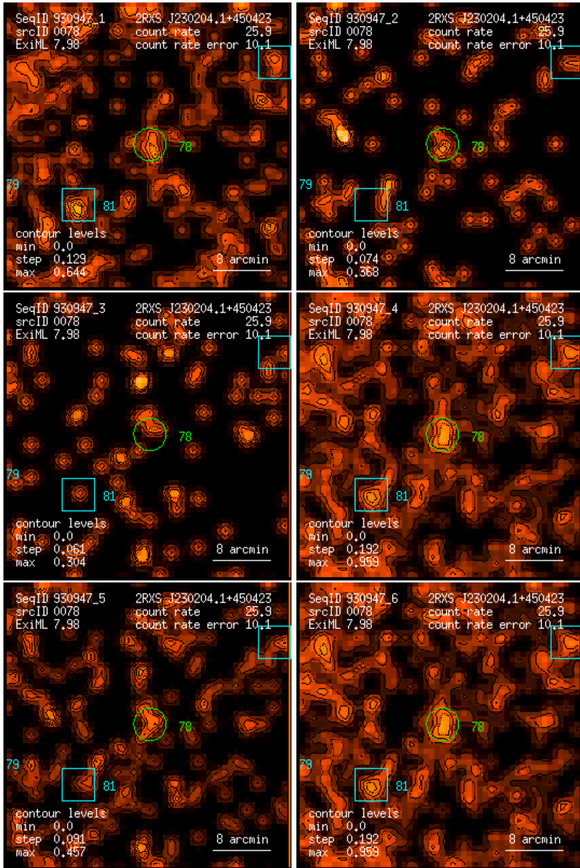
Figure 78: RASS 930947: detection 0078: band rate images, Gaussian filter: (1) PSPC channels 11 – 41, (2) 52 – 90, (3) 91 – 201, (4) 11 – 235, (5) 52 – 201, (6) 11 – 201. Broad band rates in counts/ks. Band rate contour levels in counts/ks/arcmin 2 .
