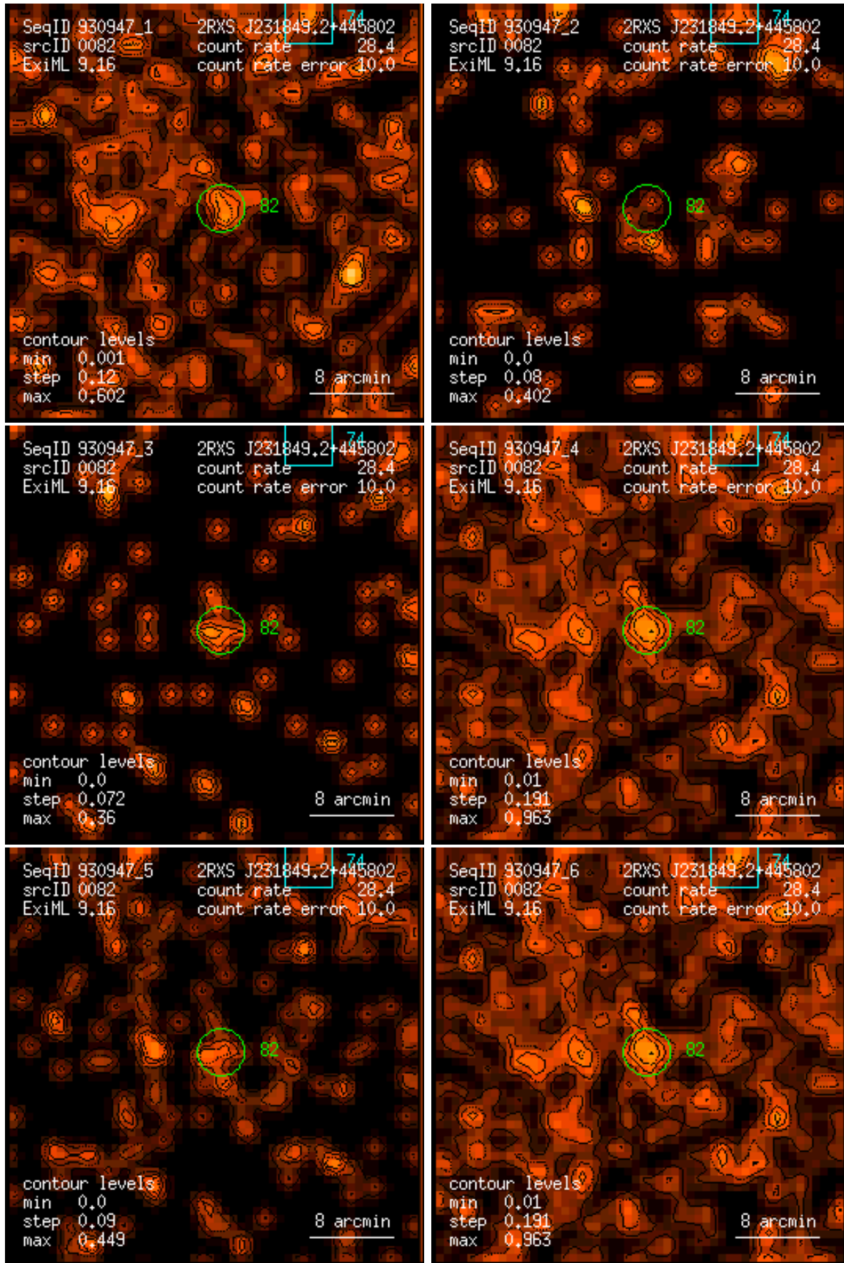
Figure 82: RASS 930947: detection 0082: band rate images, Gaussian filter: (1) PSPC channels 11 – 41, (2) 52 – 90, (3) 91 – 201, (4) 11 – 235, (5) 52 – 201, (6) 11 – 201. Broad band rates in counts/ks. Band rate contour levels in counts/ks/arcmin 2 .
