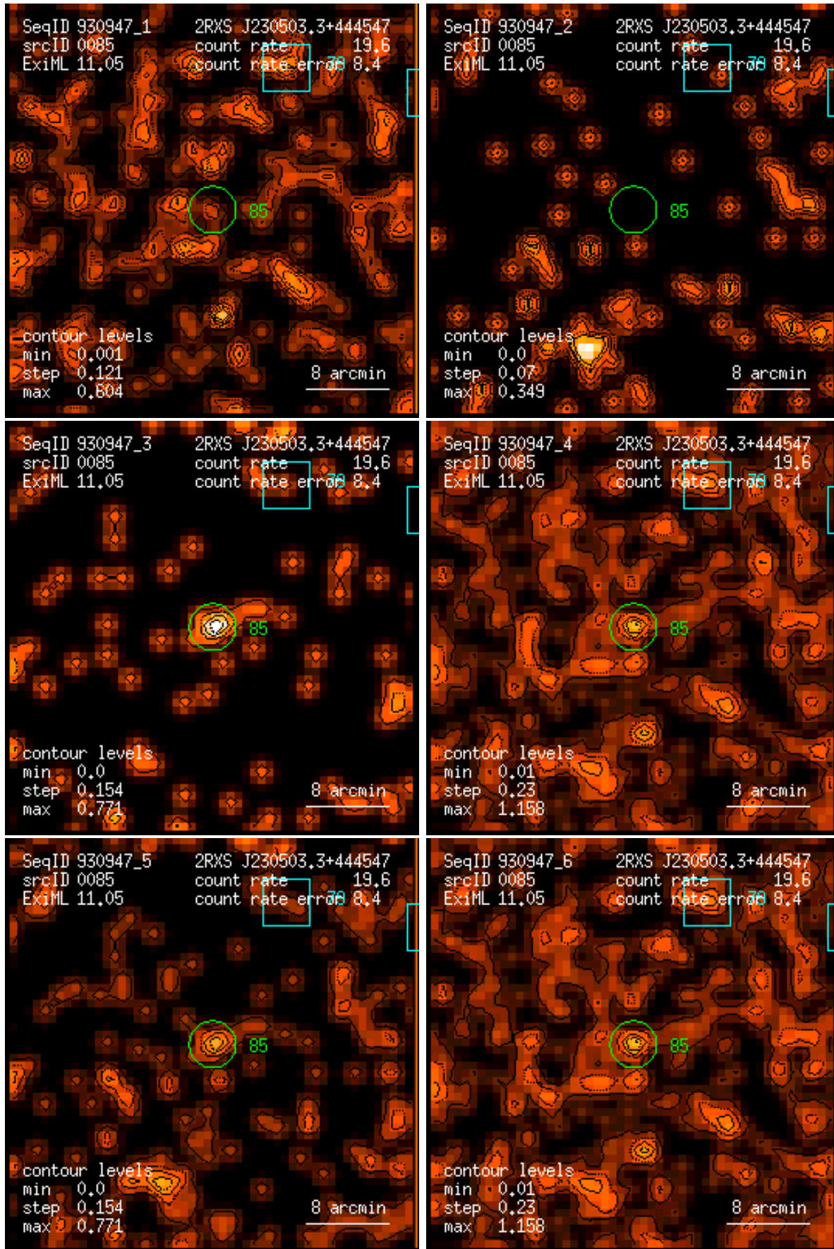
Figure 85: RASS 930947: detection 0085: band rate images, Gaussian filter: (1) PSPC channels 11 – 41, (2) 52 – 90, (3) 91 – 201, (4) 11 – 235, (5) 52 – 201, (6) 11 – 201. Broad band rates in counts/ks. Band rate contour levels in counts/ks/arcmin 2 .
