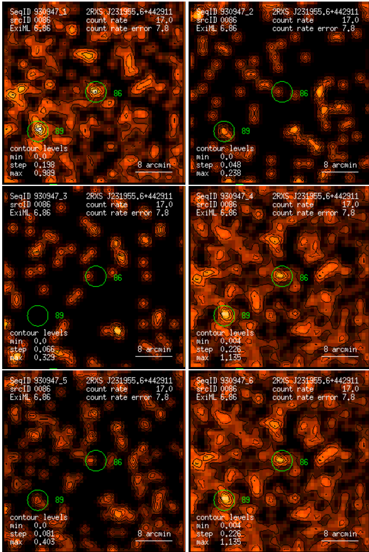
Figure 86: RASS 930947: detection 0086: band rate images, Gaussian filter: (1) PSPC channels 11 – 41, (2) 52 – 90, (3) 91 – 201, (4) 11 – 235, (5) 52 – 201, (6) 11 – 201. Broad band rates in counts/ks. Band rate contour levels in counts/ks/arcmin 2 .
