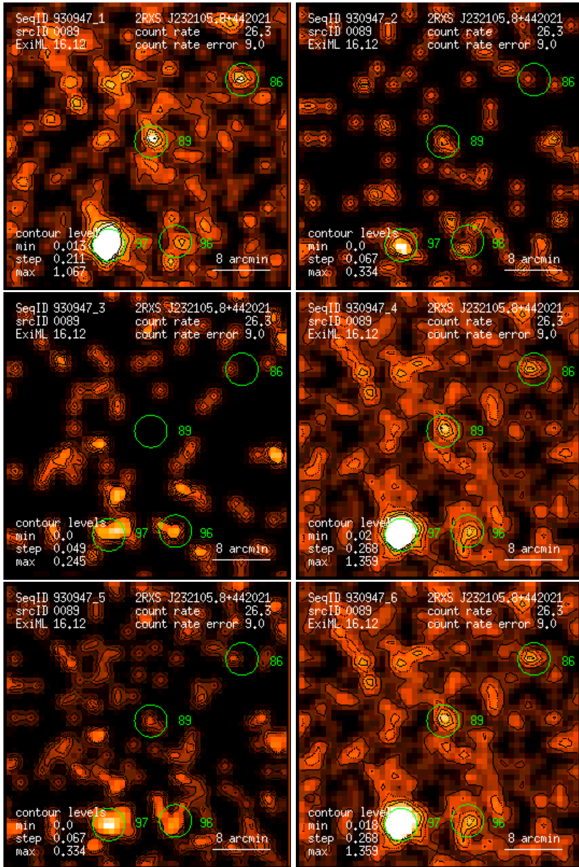
Figure 89: RASS 930947: detection 0089: band rate images, Gaussian filter: (1) PSPC channels 11 – 41, (2) 52 – 90, (3) 91 – 201, (4) 11 – 235, (5) 52 – 201, (6) 11 – 201. Broad band rates in counts/ks. Band rate contour levels in counts/ks/arcmin 2 .
