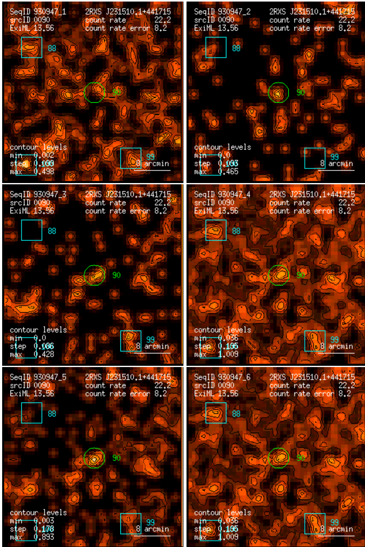
Figure 90: RASS 930947: detection 0090: band rate images, Gaussian filter: (1) PSPC channels 11 – 41, (2) 52 – 90, (3) 91 – 201, (4) 11 – 235, (5) 52 – 201, (6) 11 – 201. Broad band rates in counts/ks. Band rate contour levels in counts/ks/arcmin 2 .
