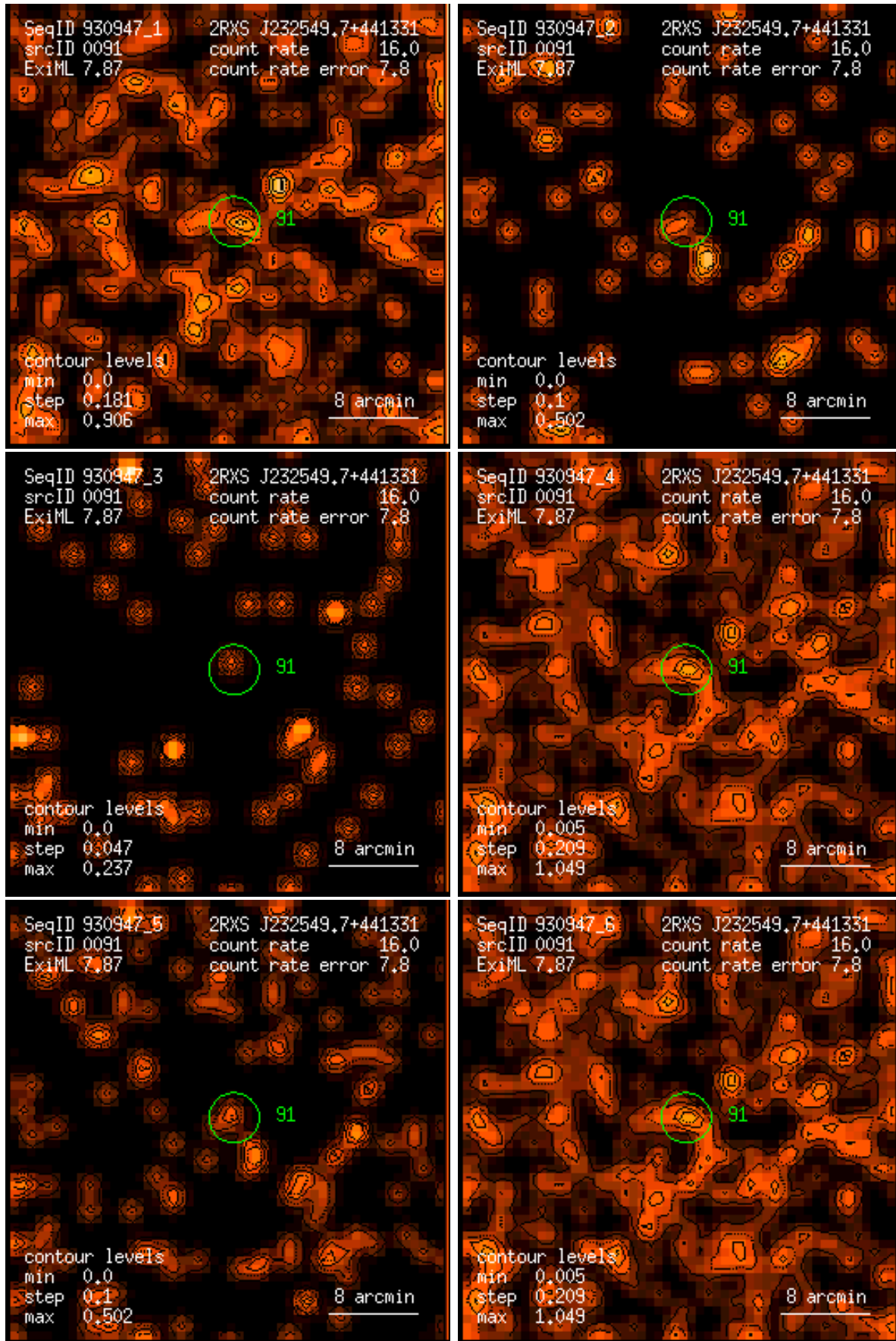
Figure 91: RASS 930947: detection 0091: band rate images, Gaussian filter: (1) PSPC channels 11 – 41, (2) 52 – 90, (3) 91 – 201, (4) 11 – 235, (5) 52 – 201, (6) 11 – 201. Broad band rates in counts/ks. Band rate contour levels in counts/ks/arcmin 2 .
