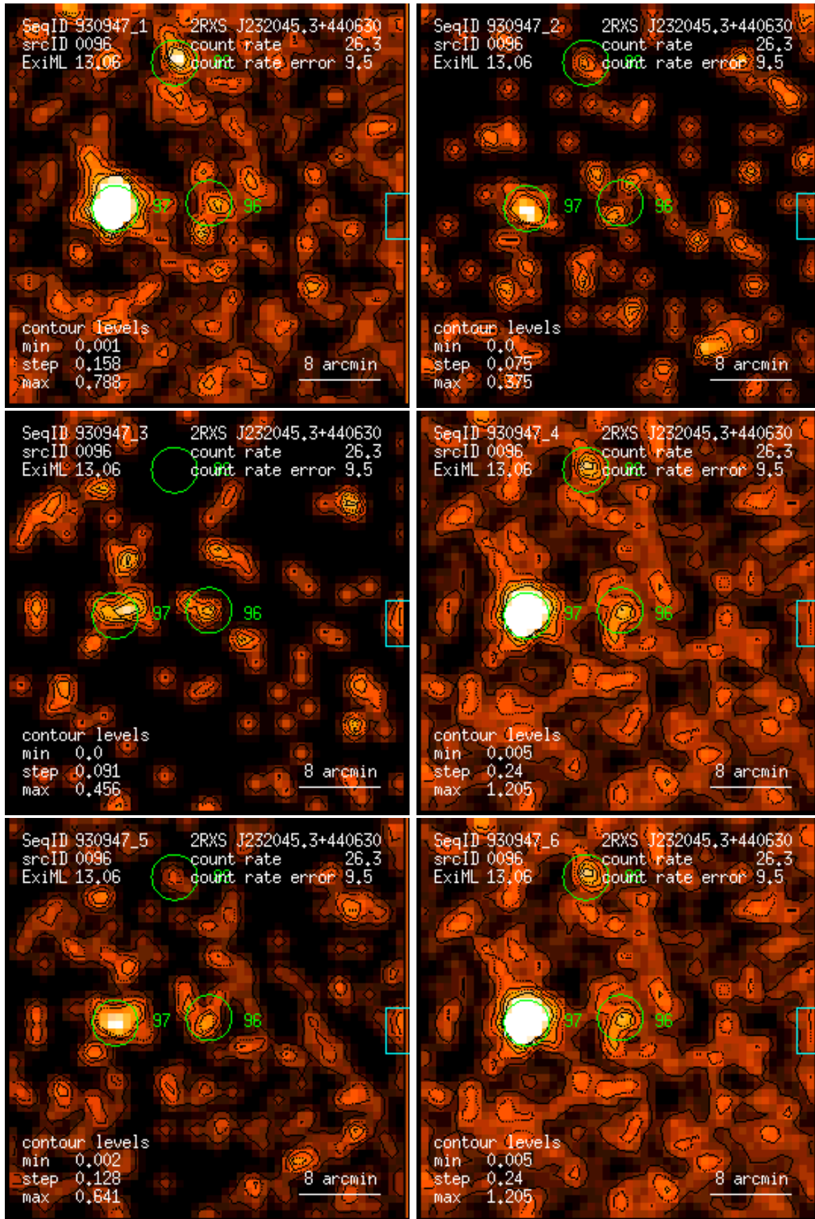
Figure 96: RASS 930947: detection 0096: band rate images, Gaussian filter: (1) PSPC channels 11 – 41, (2) 52 – 90, (3) 91 – 201, (4) 11 – 235, (5) 52 – 201, (6) 11 – 201. Broad band rates in counts/ks. Band rate contour levels in counts/ks/arcmin 2 .
