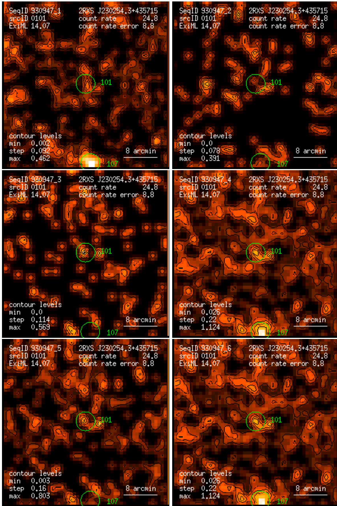
Figure 101: RASS 930947: detection 0101: band rate images, Gaussian filter: (1) PSPC channels 11 – 41, (2) 52 – 90, (3) 91 – 201, (4) 11 – 235, (5) 52 – 201, (6) 11 – 201. Broad band rates in counts/ks. Band rate contour levels in counts/ks/arcmin 2 .
