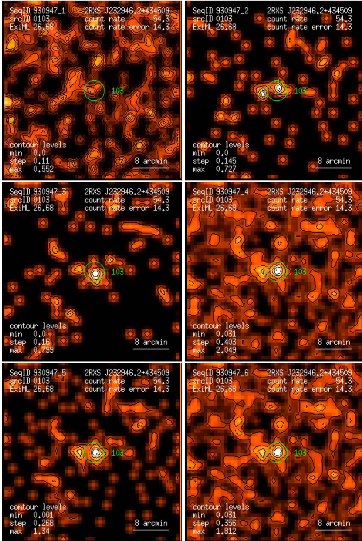
Figure 103: RASS 930947: detection 0103: band rate images, Gaussian filter: (1) PSPC channels 11 – 41, (2) 52 – 90, (3) 91 – 201, (4) 11 – 235, (5) 52 – 201, (6) 11 – 201. Broad band rates in counts/ks. Band rate contour levels in counts/ks/arcmin 2 .
