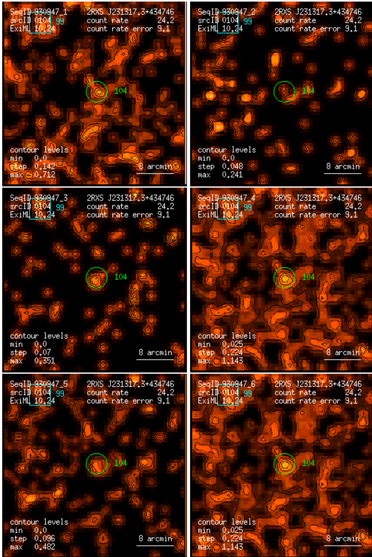
Figure 104: RASS 930947: detection 0104: band rate images, Gaussian filter: (1) PSPC channels 11 – 41, (2) 52 – 90, (3) 91 – 201, (4) 11 – 235, (5) 52 – 201, (6) 11 – 201. Broad band rates in counts/ks. Band rate contour levels in counts/ks/arcmin 2 .
