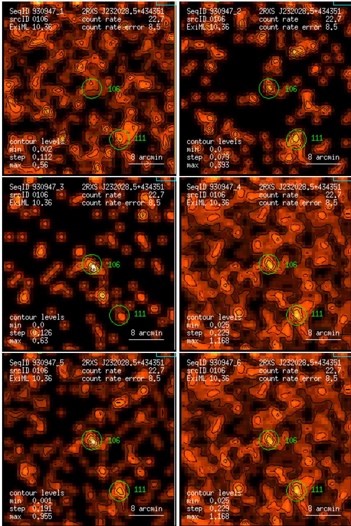
Figure 106: RASS 930947: detection 0106: band rate images, Gaussian filter: (1) PSPC channels 11 – 41, (2) 52 – 90, (3) 91 – 201, (4) 11 – 235, (5) 52 – 201, (6) 11 – 201. Broad band rates in counts/ks. Band rate contour levels in counts/ks/arcmin 2 .
