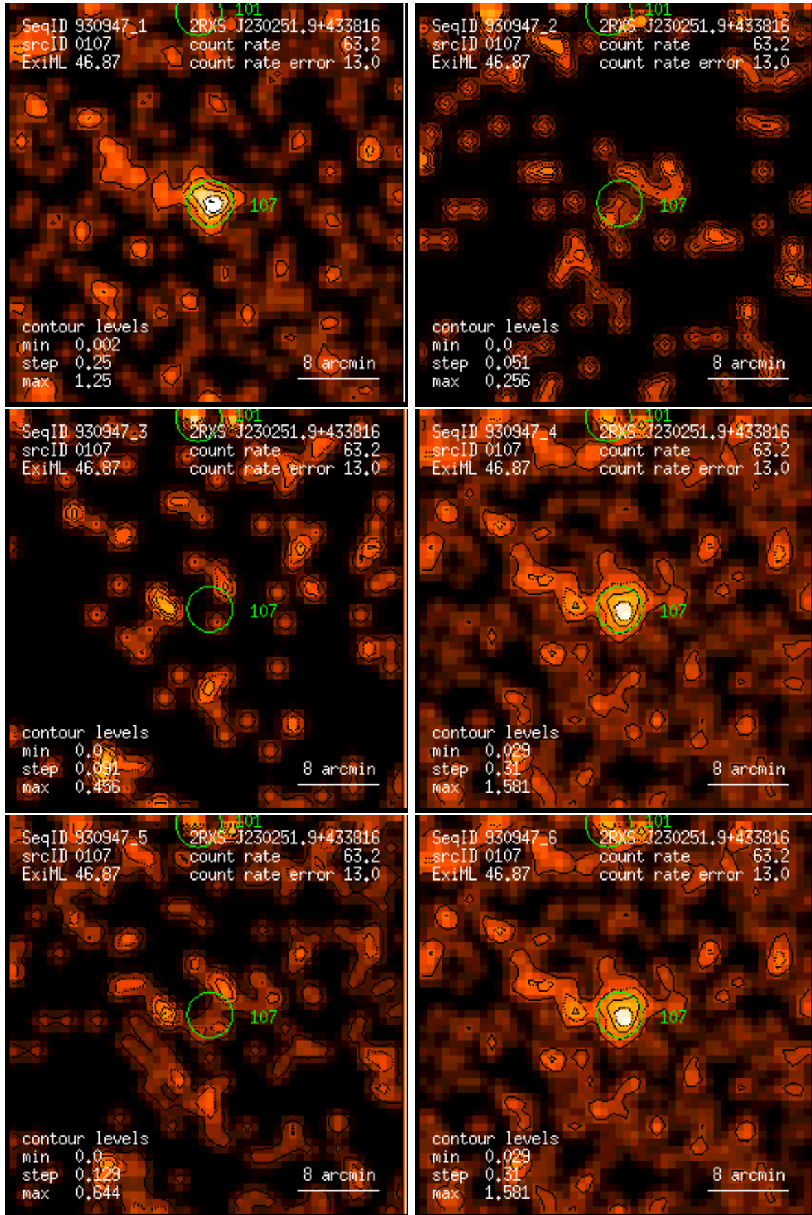
Figure 107: RASS 930947: detection 0107: band rate images, Gaussian filter: (1) PSPC channels 11 – 41, (2) 52 – 90, (3) 91 – 201, (4) 11 – 235, (5) 52 – 201, (6) 11 – 201. Broad band rates in counts/ks. Band rate contour levels in counts/ks/arcmin 2 .
