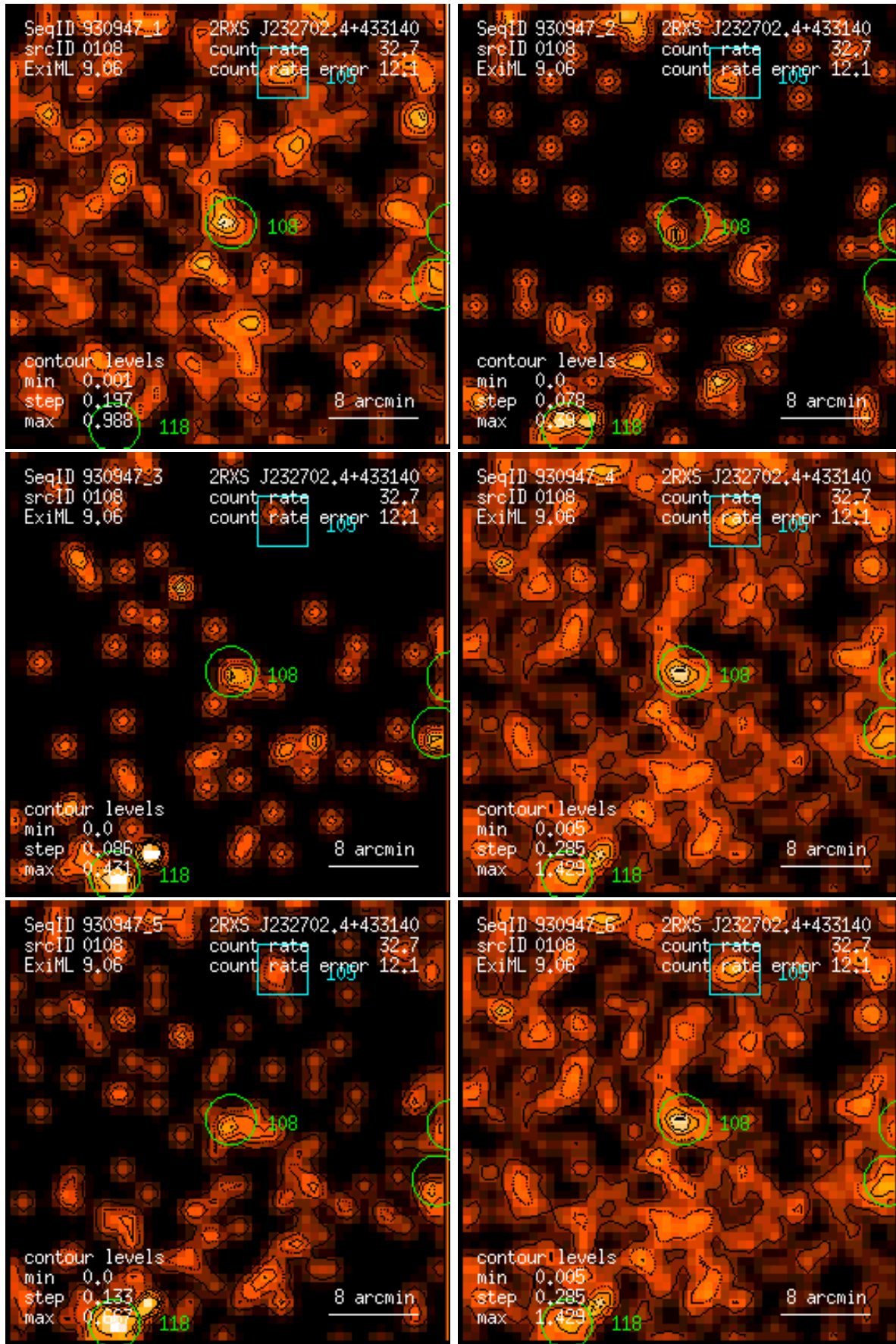
Figure 108: RASS 930947: detection 0108: band rate images, Gaussian filter: (1) PSPC channels 11 – 41, (2) 52 – 90, (3) 91 – 201, (4) 11 – 235, (5) 52 – 201, (6) 11 – 201. Broad band rates in counts/ks. Band rate contour levels in counts/ks/arcmin 2 .
