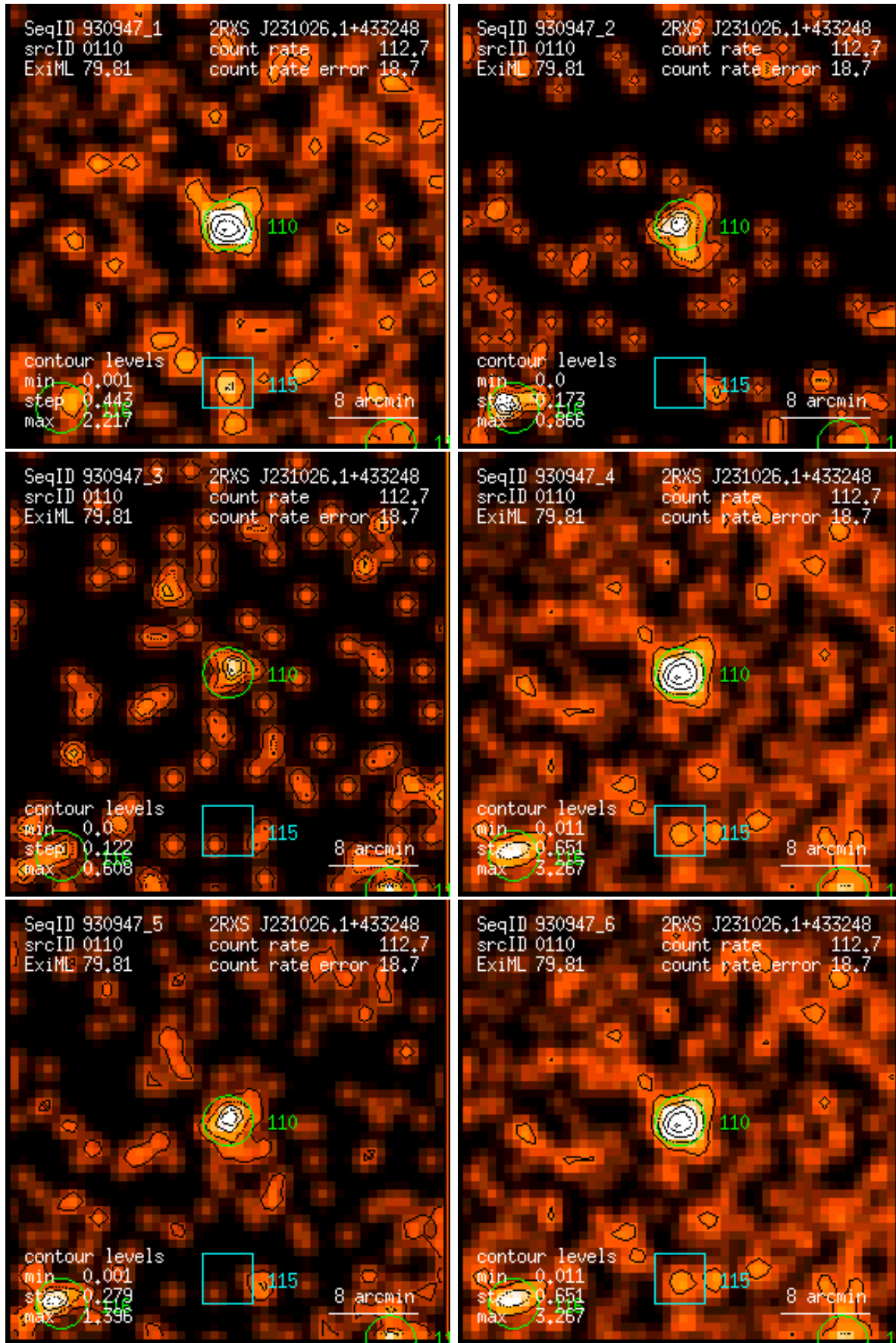
Figure 110: RASS 930947: detection 0110: band rate images, Gaussian filter: (1) PSPC channels 11 – 41, (2) 52 – 90, (3) 91 – 201, (4) 11 – 235, (5) 52 – 201, (6) 11 – 201. Broad band rates in counts/ks. Band rate contour levels in counts/ks/arcmin 2 .
