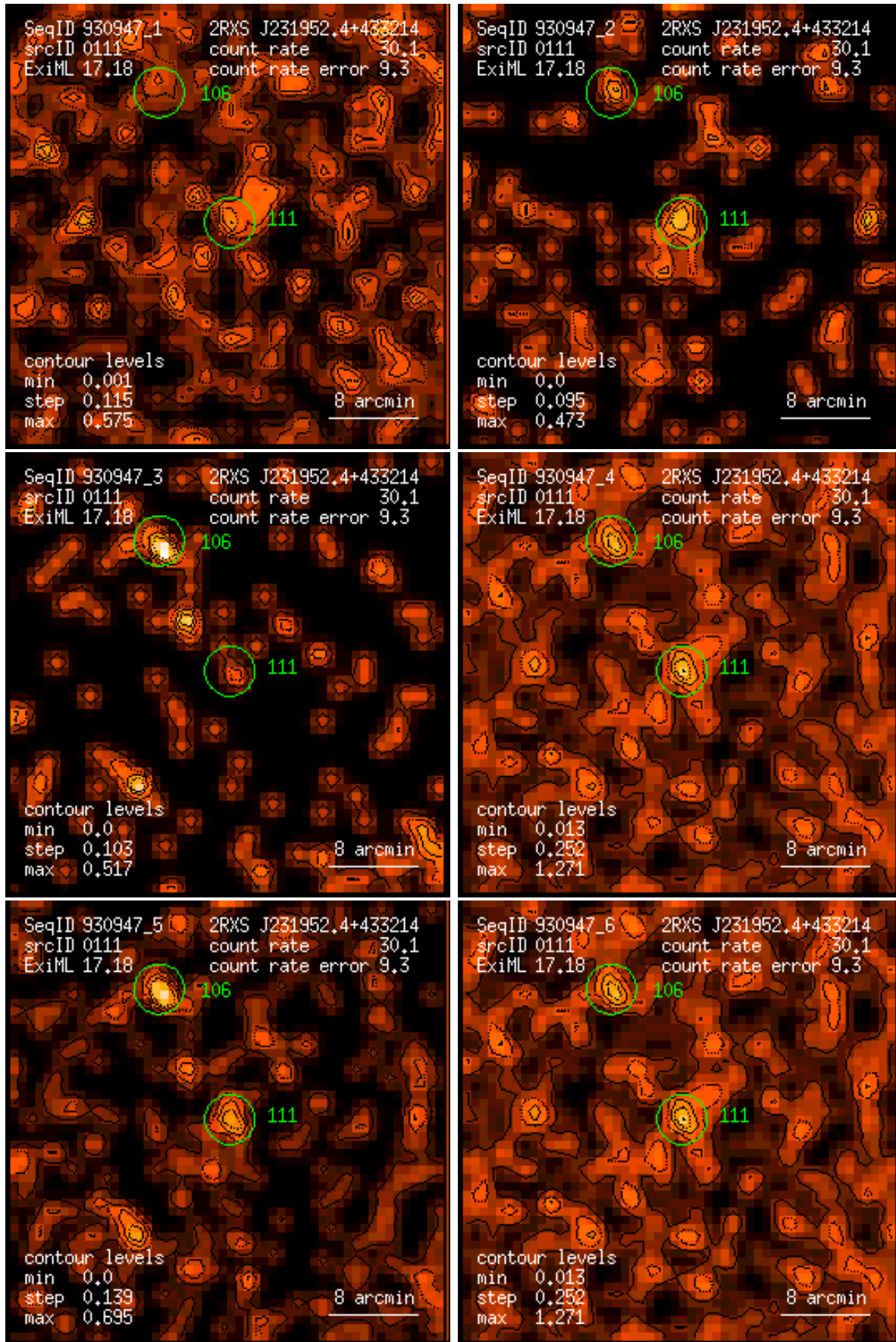
Figure 111: RASS 930947: detection 0111: band rate images, Gaussian filter: (1) PSPC channels 11 – 41, (2) 52 – 90, (3) 91 – 201, (4) 11 – 235, (5) 52 – 201, (6) 11 – 201. Broad band rates in counts/ks. Band rate contour levels in counts/ks/arcmin 2 .
