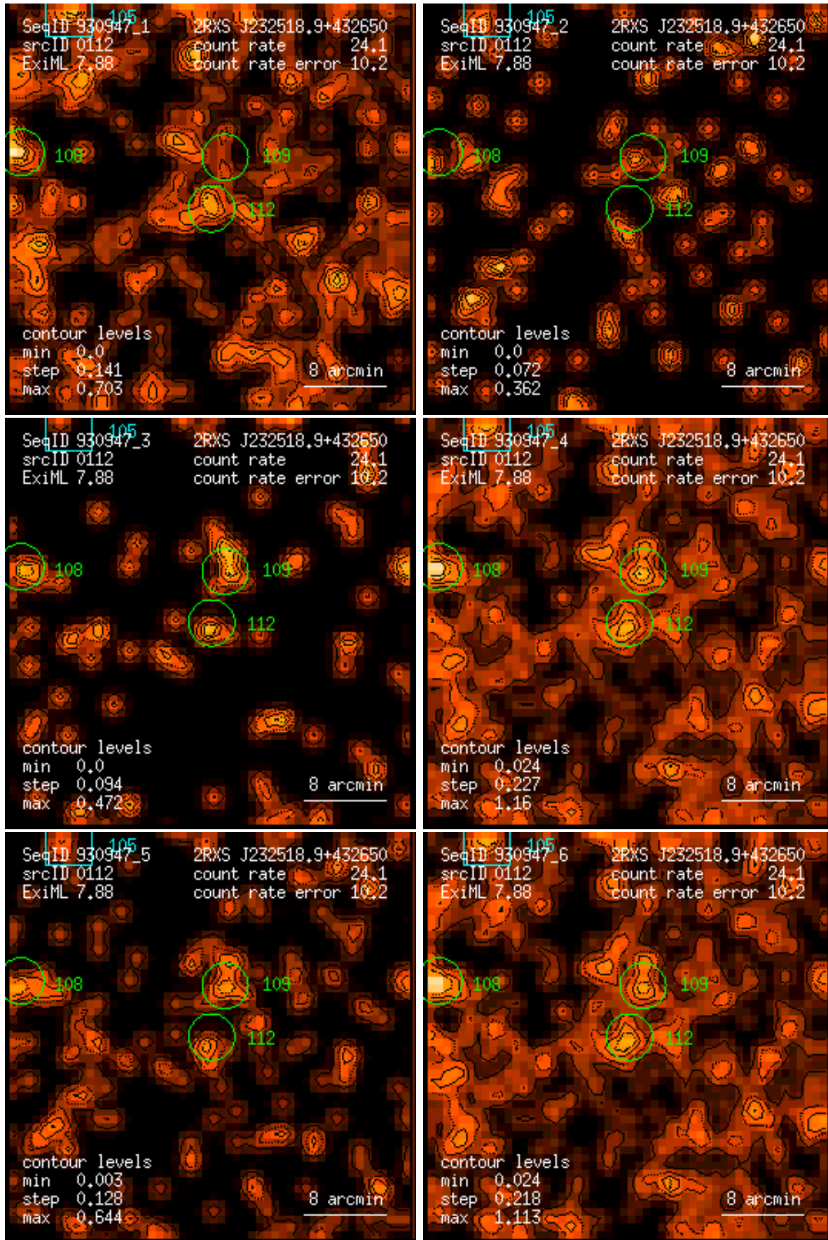
Figure 112: RASS 930947: detection 0112: band rate images, Gaussian filter: (1) PSPC channels 11 – 41, (2) 52 – 90, (3) 91 – 201, (4) 11 – 235, (5) 52 – 201, (6) 11 – 201. Broad band rates in counts/ks. Band rate contour levels in counts/ks/arcmin 2 .
