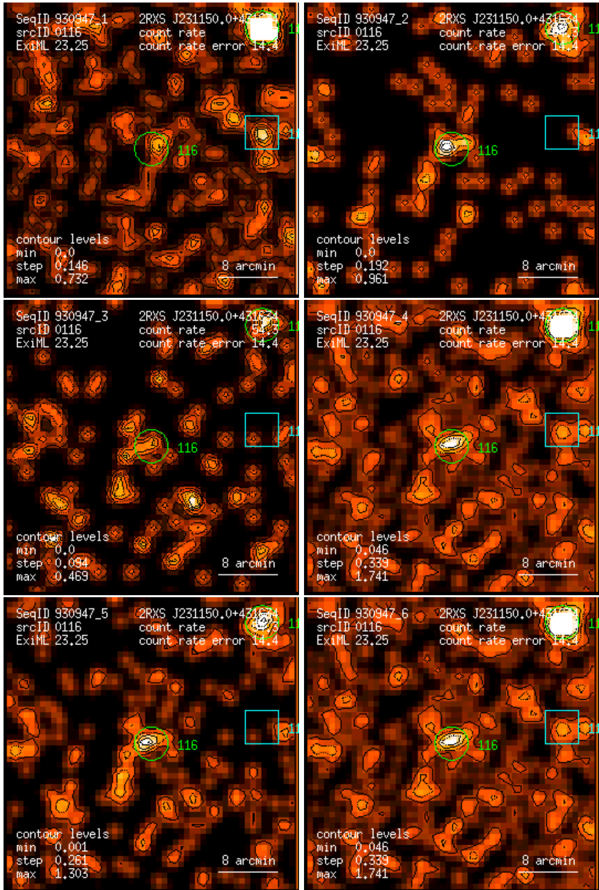
Figure 116: RASS 930947: detection 0116: band rate images, Gaussian filter: (1) PSPC channels 11 – 41, (2) 52 – 90, (3) 91 – 201, (4) 11 – 235, (5) 52 – 201, (6) 11 – 201. Broad band rates in counts/ks. Band rate contour levels in counts/ks/arcmin 2 .
