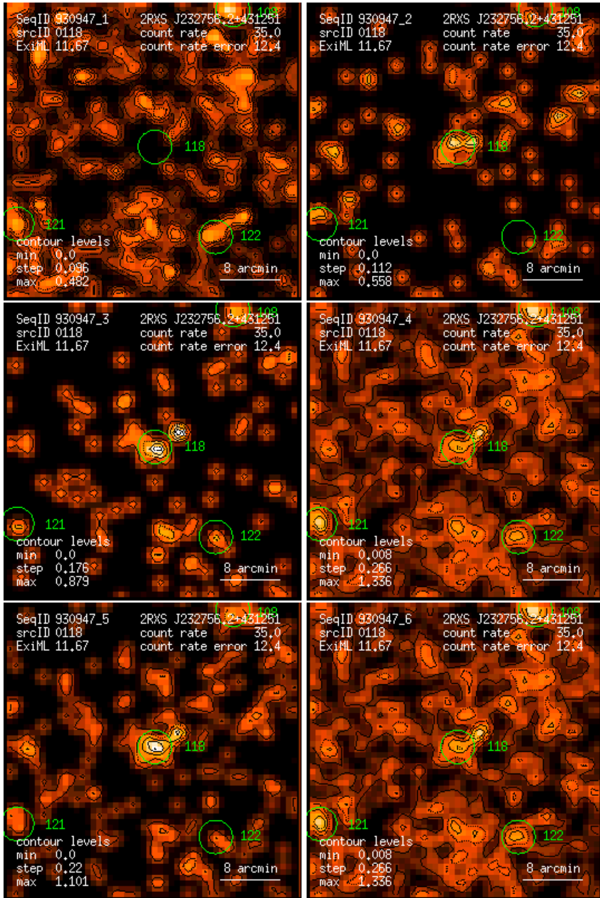
Figure 118: RASS 930947: detection 0118: band rate images, Gaussian filter: (1) PSPC channels 11 – 41, (2) 52 – 90, (3) 91 – 201, (4) 11 – 235, (5) 52 – 201, (6) 11 – 201. Broad band rates in counts/ks. Band rate contour levels in counts/ks/arcmin 2 .
