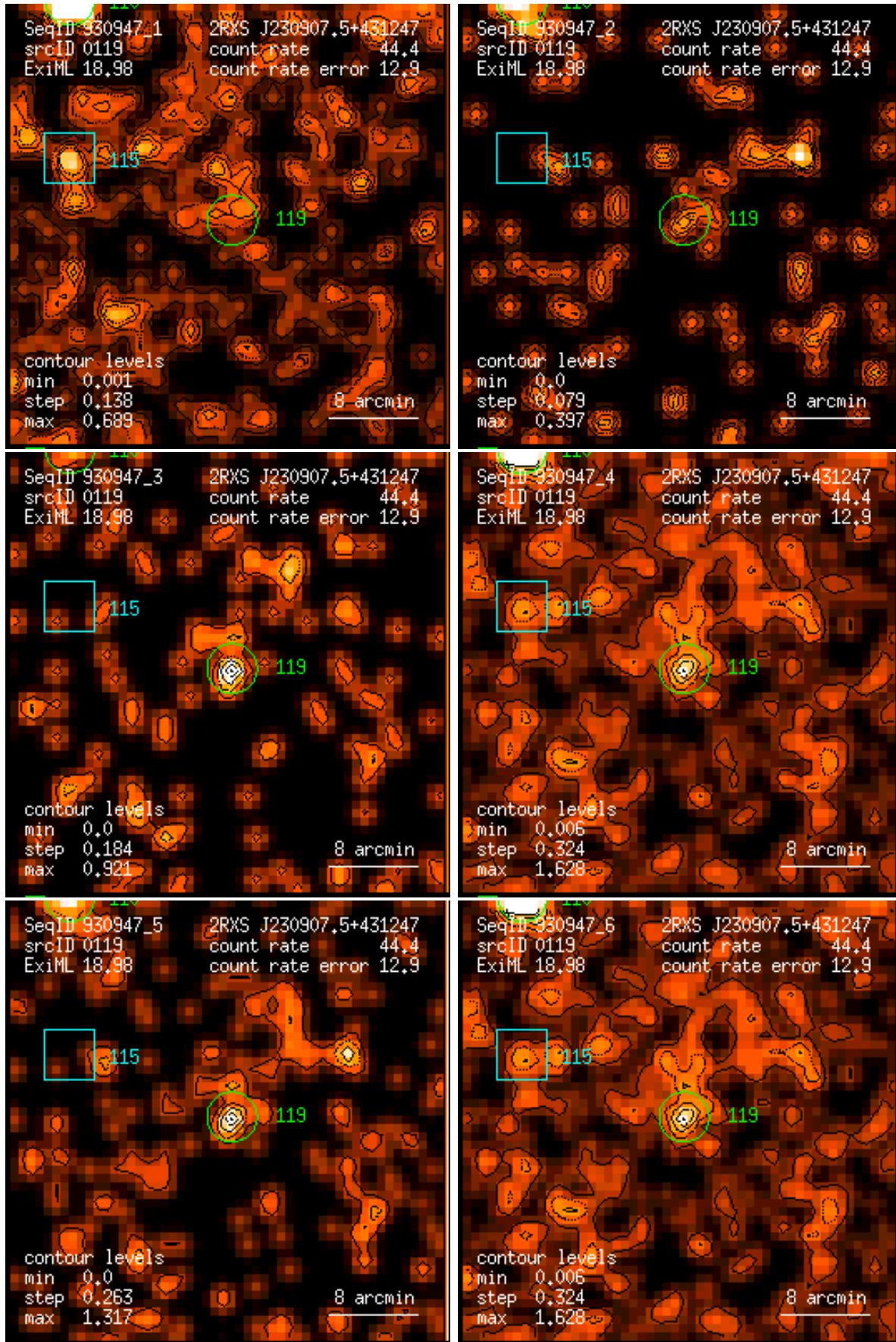
Figure 119: RASS 930947: detection 0119: band rate images, Gaussian filter: (1) PSPC channels 11 – 41, (2) 52 – 90, (3) 91 – 201, (4) 11 – 235, (5) 52 – 201, (6) 11 – 201. Broad band rates in counts/ks. Band rate contour levels in counts/ks/arcmin 2 .
