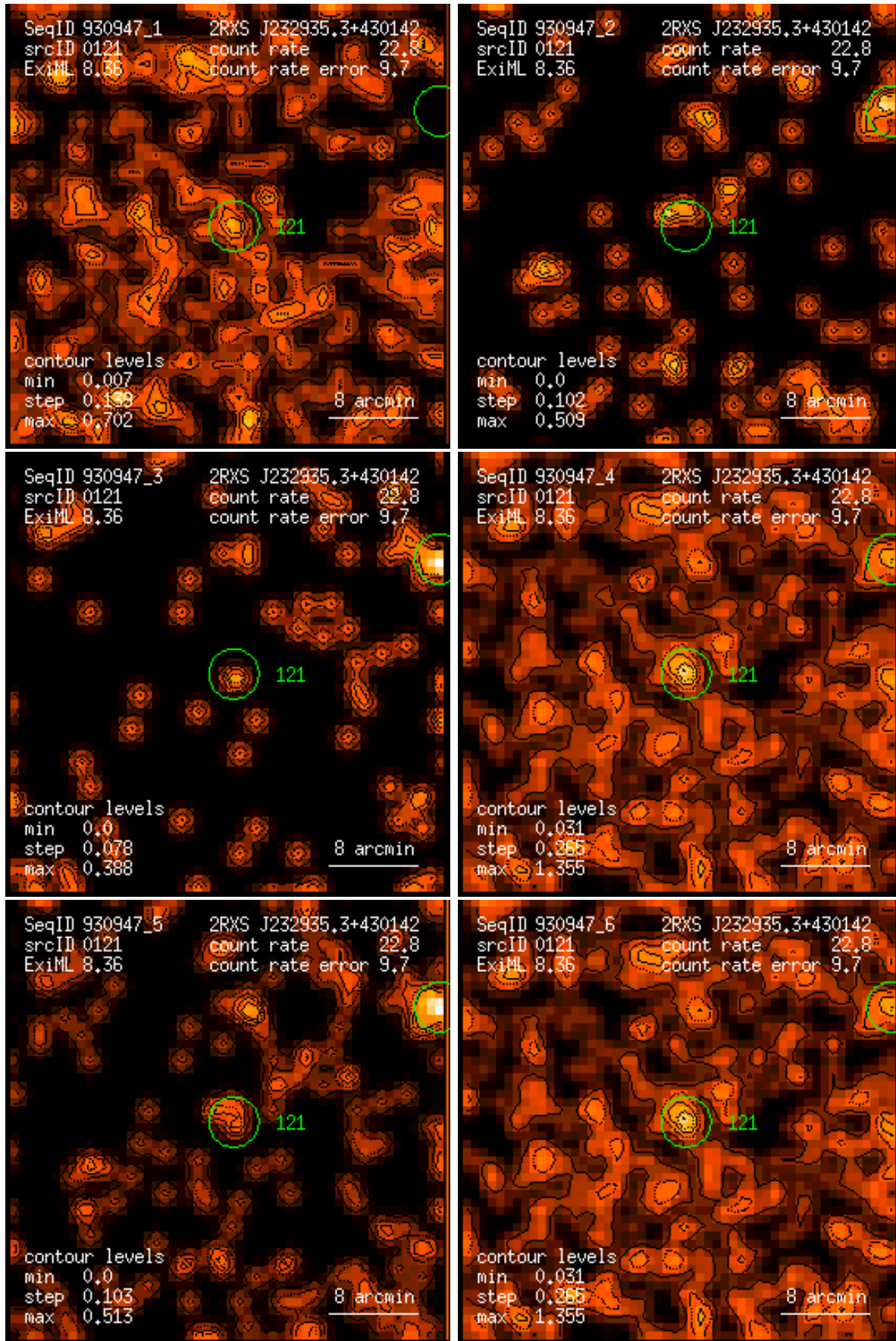
Figure 121: RASS 930947: detection 0121: band rate images, Gaussian filter: (1) PSPC channels 11 – 41, (2) 52 – 90, (3) 91 – 201, (4) 11 – 235, (5) 52 – 201, (6) 11 – 201. Broad band rates in counts/ks. Band rate contour levels in counts/ks/arcmin 2 .
