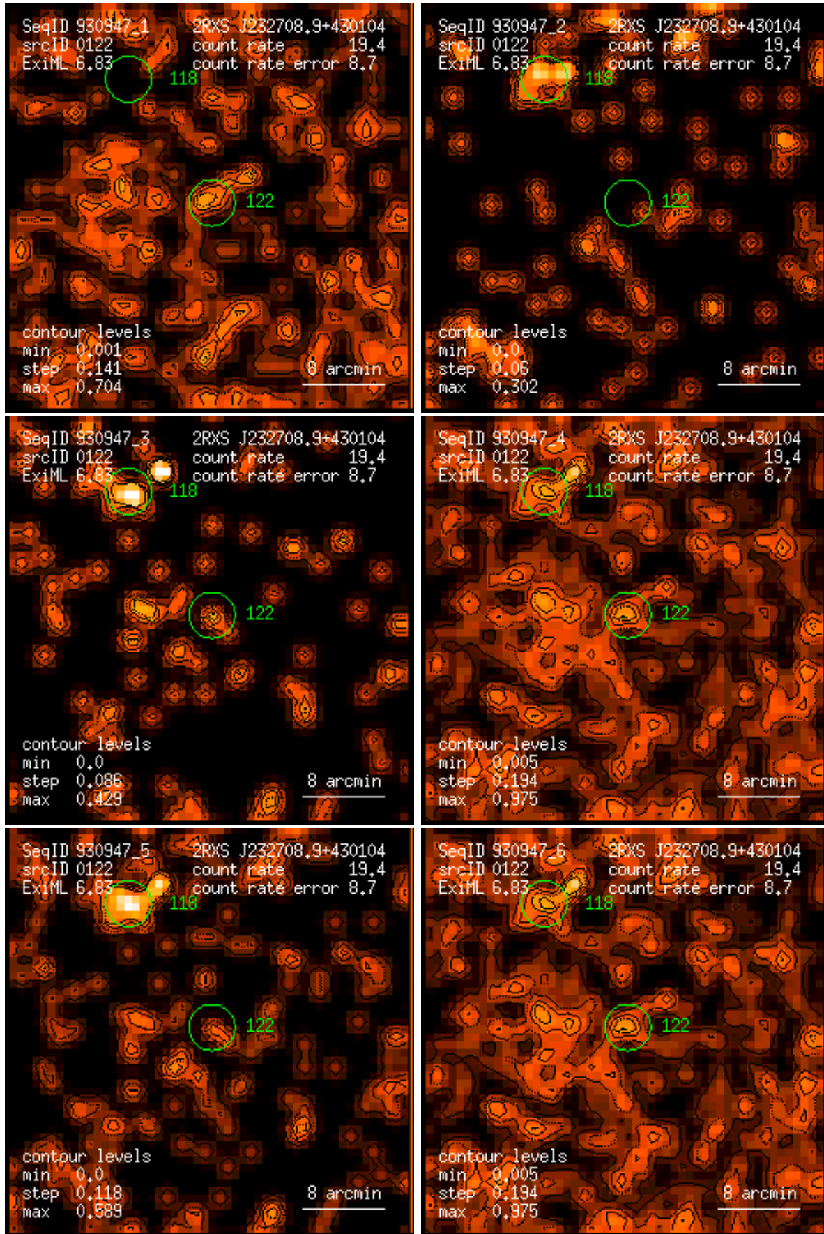
Figure 122: RASS 930947: detection 0122: band rate images, Gaussian filter: (1) PSPC channels 11 – 41, (2) 52 – 90, (3) 91 – 201, (4) 11 – 235, (5) 52 – 201, (6) 11 – 201. Broad band rates in counts/ks. Band rate contour levels in counts/ks/arcmin 2 .
