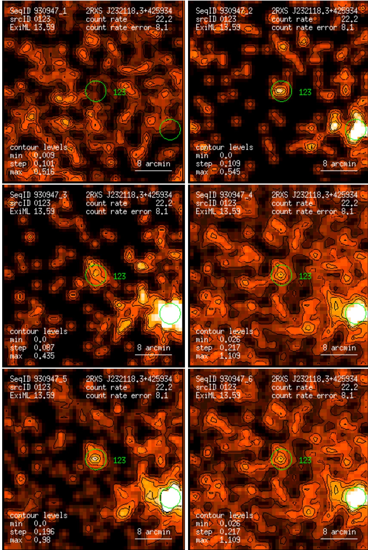
Figure 123: RASS 930947: detection 0123: band rate images, Gaussian filter: (1) PSPC channels 11 – 41, (2) 52 – 90, (3) 91 – 201, (4) 11 – 235, (5) 52 – 201, (6) 11 – 201. Broad band rates in counts/ks. Band rate contour levels in counts/ks/arcmin 2 .
