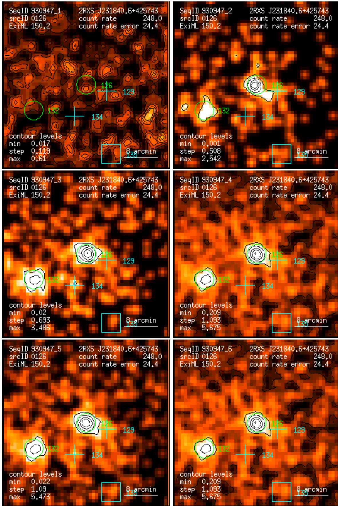
Figure 126: RASS 930947: detection 0126: band rate images, Gaussian filter: (1) PSPC channels 11 – 41, (2) 52 – 90, (3) 91 – 201, (4) 11 – 235, (5) 52 – 201, (6) 11 – 201. Broad band rates in counts/ks. Band rate contour levels in counts/ks/arcmin 2 .
