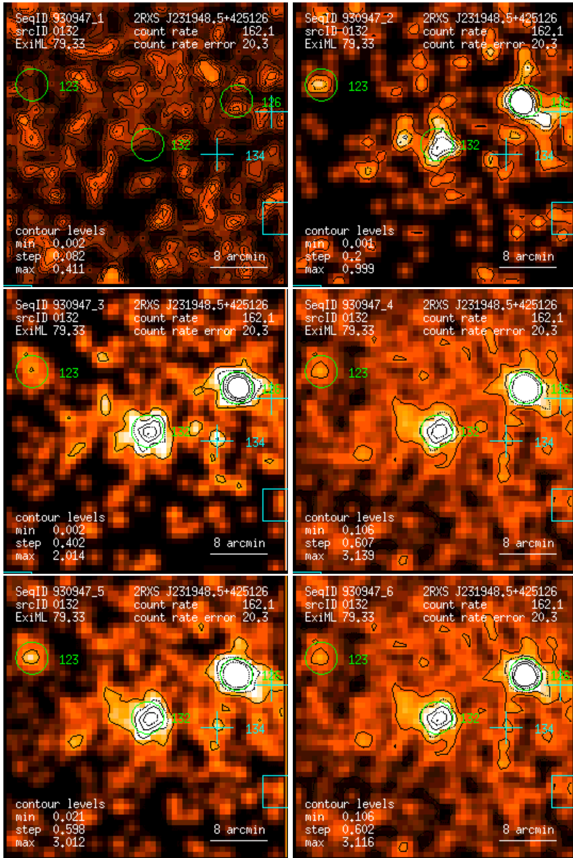
Figure 132: RASS 930947: detection 0132: band rate images, Gaussian filter: (1) PSPC channels 11 – 41, (2) 52 – 90, (3) 91 – 201, (4) 11 – 235, (5) 52 – 201, (6) 11 – 201. Broad band rates in counts/ks. Band rate contour levels in counts/ks/arcmin 2 .
