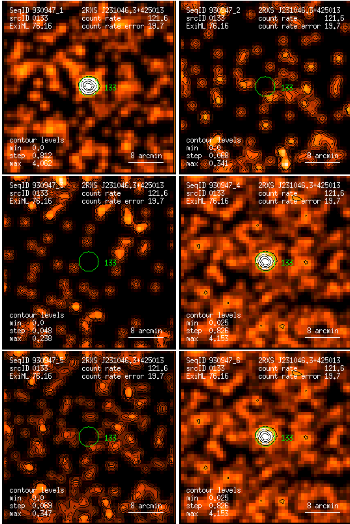
Figure 133: RASS 930947: detection 0133: band rate images, Gaussian filter: (1) PSPC channels 11 – 41, (2) 52 – 90, (3) 91 – 201, (4) 11 – 235, (5) 52 – 201, (6) 11 – 201. Broad band rates in counts/ks. Band rate contour levels in counts/ks/arcmin 2 .
